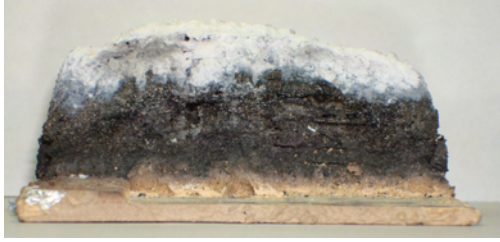
Fig. 9. Intumescent layer cross section cut. Reference and position of the thermocouples.
