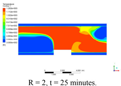
Fig. 17 - Contour of the global temperature for the compartment C1 considering the steel beam IPE600 for two relative positions of a class 3 fire event.
