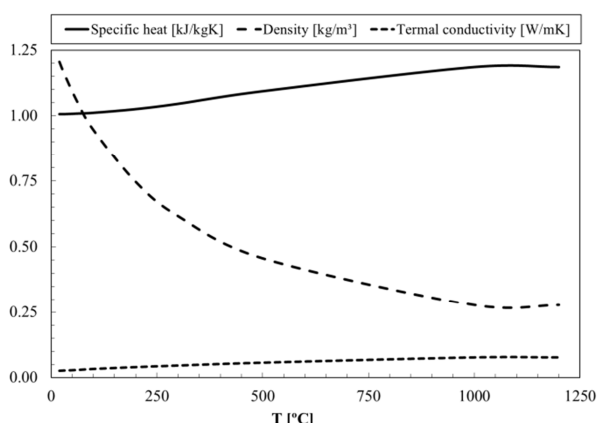
Fig. 7 - Properties of the air.
