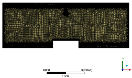
Fig. 10 - The mesh used in the CFD simulation corresponding for compartment of fire 1.
