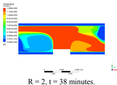
Fig. 17 - Contour of the global temperature for the compartment C1 considering the steel beam IPE600 for two relative positions of a class 3 fire event.
