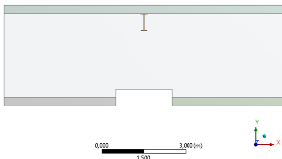
Fig. 9 - The geometry used in the CFD simulation corresponding for compartment of fire 1.
