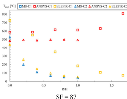
Fig. 16 - Maximum temperatures in the steel beam, considering the fire event (class 3) in both compartments C1 and C2. Solution methods: - simple calc. methods (MS and Elefir-EN), advanced calc. method (ANSYS).
