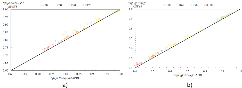
Figure 3: Comparison results between the numerical simulation and improved formulae for the calculations of the resistance to axial compression (a) and effective flexural stiffness around the weak axis (b).
