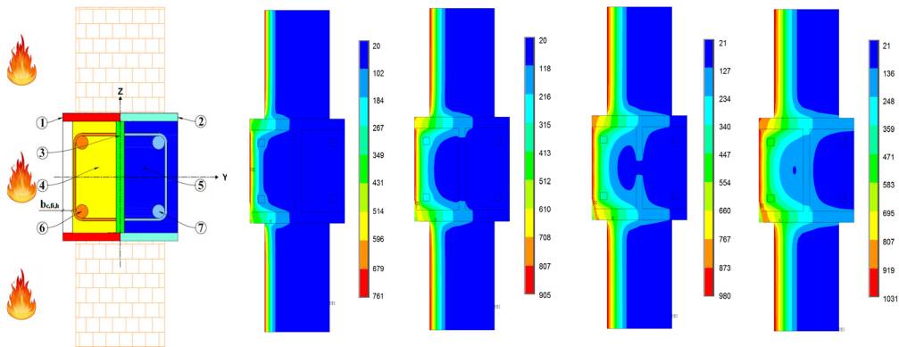
Figure 2: Temperature distribution in four times of resistance and results obtained.
