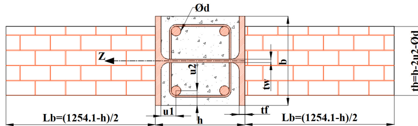
Figure 1: Partially encased column embedded on wall.
