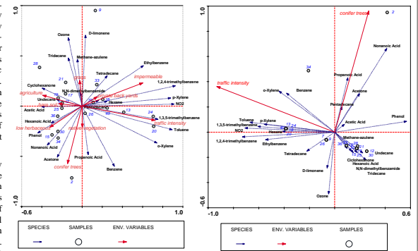
Figure 6. Triplot of PCA with samples, pollutants and environmental variables.
