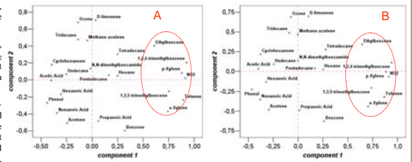
Figure 5. Loading Plots (unrotated pattern (A) and varimax rotation (B)) for the first two components.
