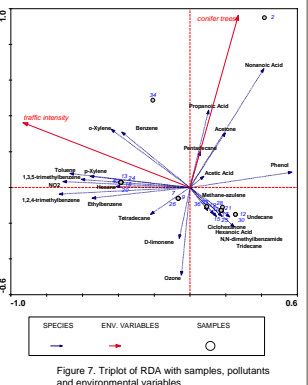
Figure 7. Triplot of RDA with samples, pollutants and environmental variables.
