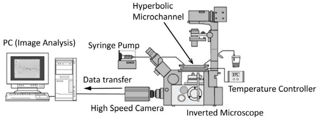
Figure 2: Experimental set-up consisting of an inverted microscope (IX71, Olympus, Japan), a high speed camera (Phantom v7.1, Vision Research, USA), a syringe pump (KD Scientific Inc., USA) and a thermo plate controller (Tokai Hit, Japan).
