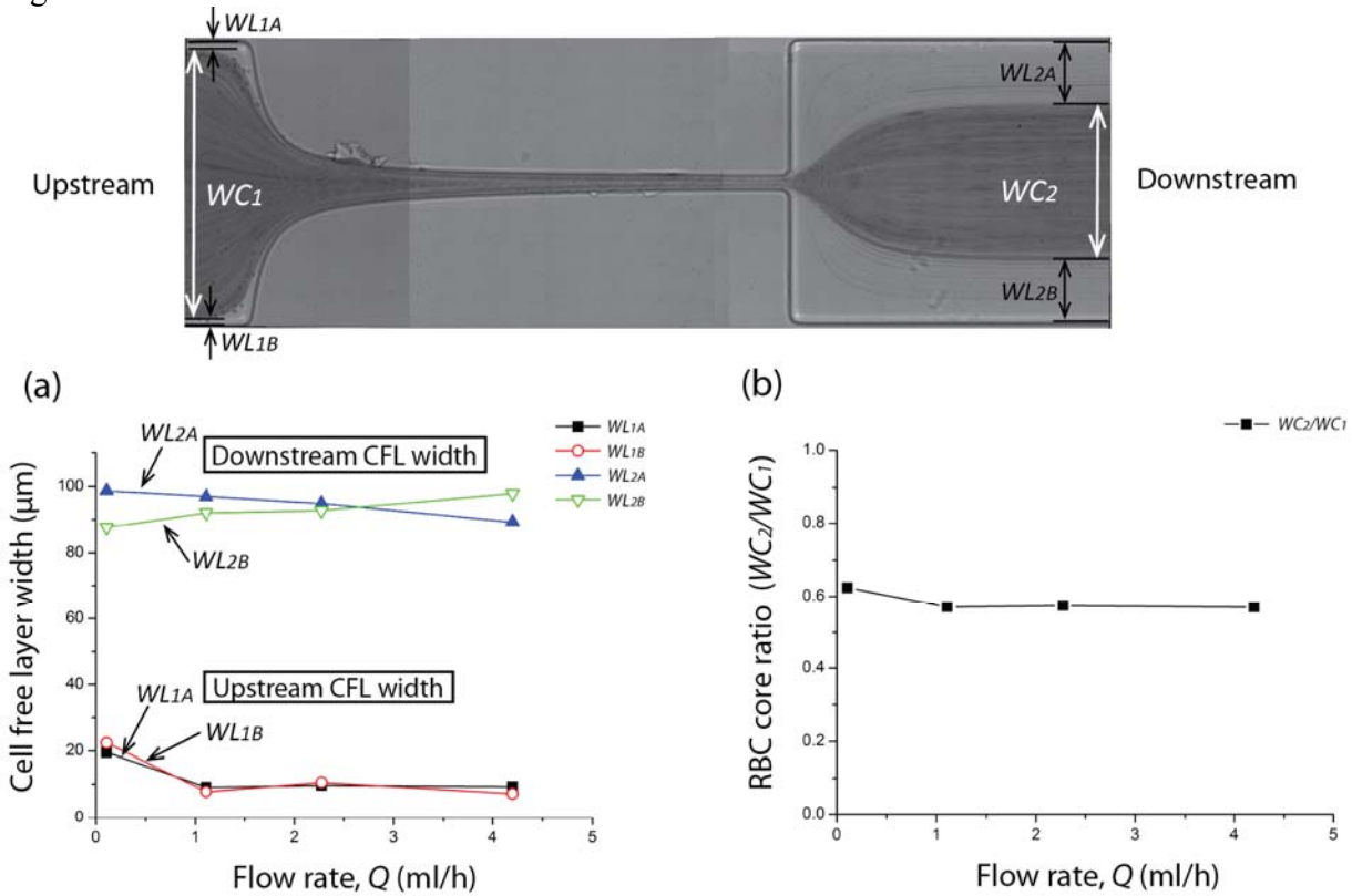
Figure 9 Cell free layer measurements. (a) Width of CFLs upstream and downstream as a function of the flow rate: Q = 0.11\text{ml/h} , Q = 1.11\text{ml/h} , Q = 2.27\text{ml/h} and Q = 4.2\text{ml/h} . (b) Effect of the flow rate on the ratio of the core RBC widths downstream and upstream of the contraction.
