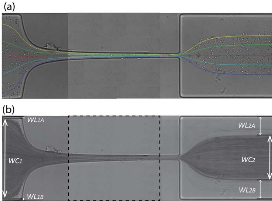
Figure 5. a) RBC trajectories manually tracked by MTrackJ plug-in from ImageJ. b) Image obtained after post-processing using the minimum intensity level option in ImageJ, Z_{project} operation for the measurement of the cell free layer and relevant variables: WC_1 and WC_2 are the widths of RBC core upstream and downstream of the hyperbolic region, respectively. WL_{1A} and WL_{1B} are the widths of CFL upstream of the contraction region, and WL_{2A} and WL_{2B} are the widths of CFL downstream of the contraction region. Each image is a combination of three separate images covering different parts of the channel. The dashed lines indicate the boundaries between images.
