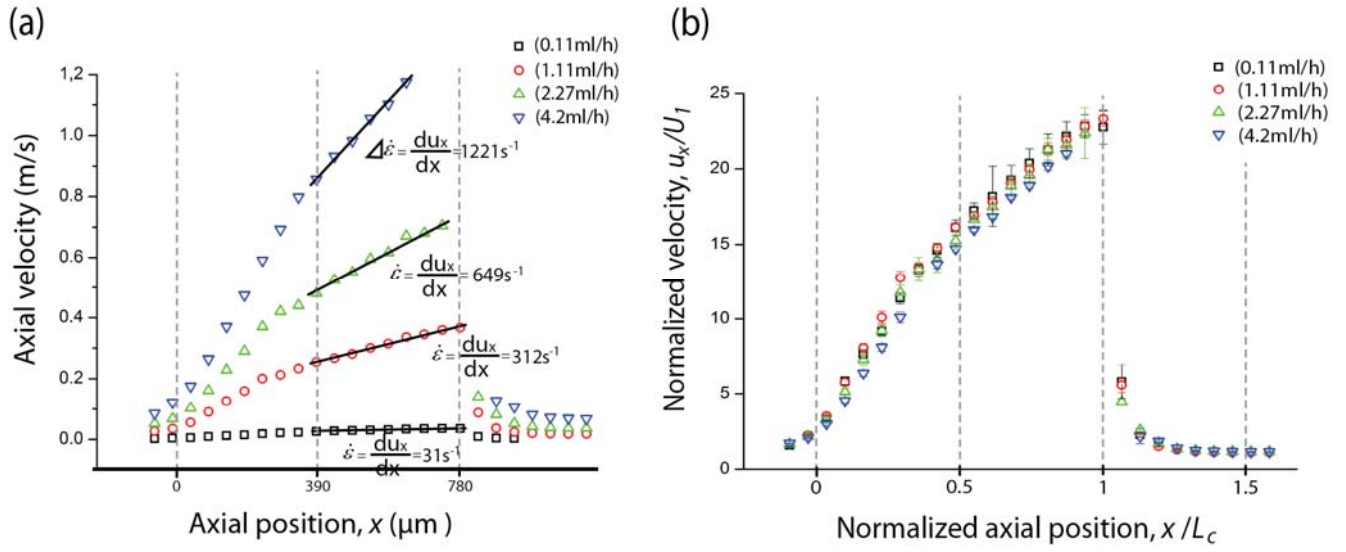
Figure 6. a) Axial velocity profiles of flowing RBCs along the centerline for four flow rates ( Q=0.11 ml/h, Q=1.11 ml/h, Q=2.27 ml/h and Q=4.2 ml/h). The solid lines represent the fit used to determine the strain rate in the linear region, calculated from the slope du_x/dx . b) Normalized axial velocity profile u_x/U_1 , where u_x refers to an instantaneous cell velocity average, and U_1 is the cross-section overall mean velocity based on the large channel, U_1 = Q/(d W_1) . The dashed lines indicate the start ( x/L_c = 0 ), mid ( x/L_c = 0.5 ) and end ( x/L_c = 1 ) of the contraction region.
