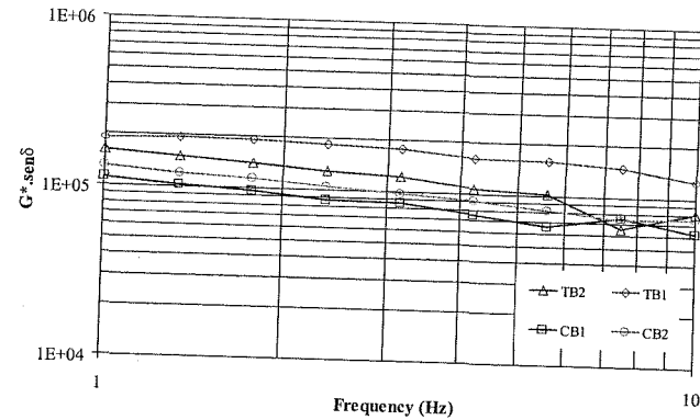
Figure 8. G^* \cdot \sin\delta at 20°C
