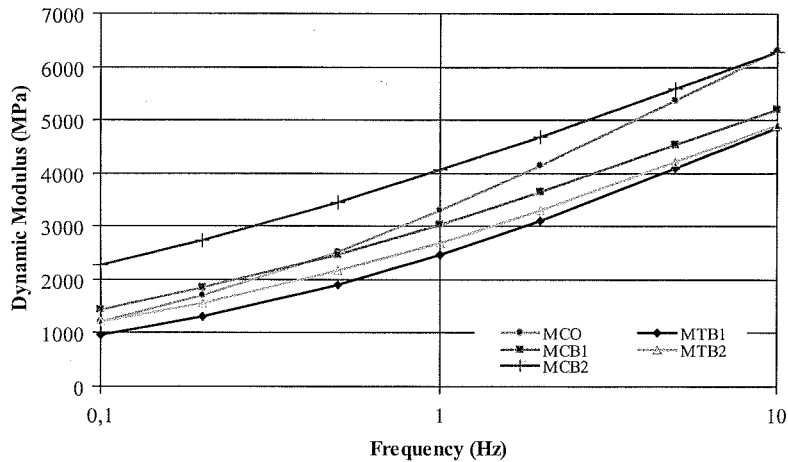
Figure 11. Dynamic modulus of the mixtures
