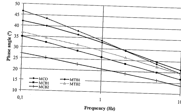
Figure 12. Phase angle of the mixtures
