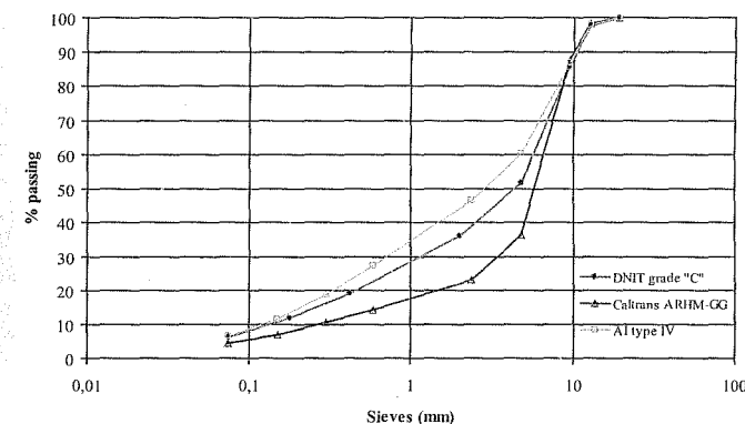
Figure 1. Aggregate gradations
