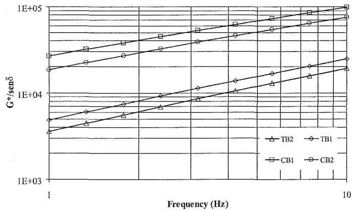
Figure 7. G^*/\sin\delta at 60°C
