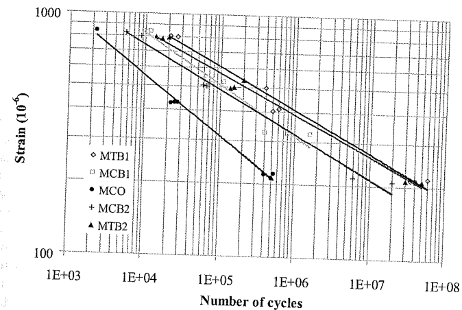
Figure 13. Fatigue curves
