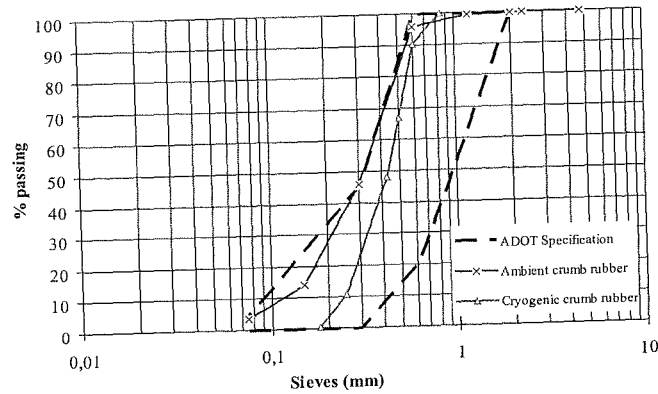
Figure 2. Crumb rubber gradations
