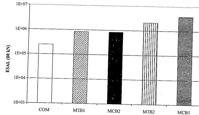
Figure 15. Permanent deformation results
