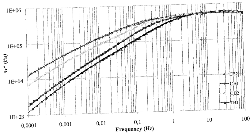
Figure 10. Master curves of the asphalt rubber binders
