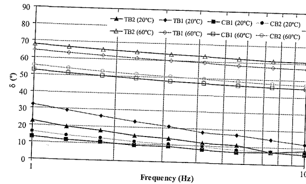
Figure 9. Asphalts rubber binder phase angles
