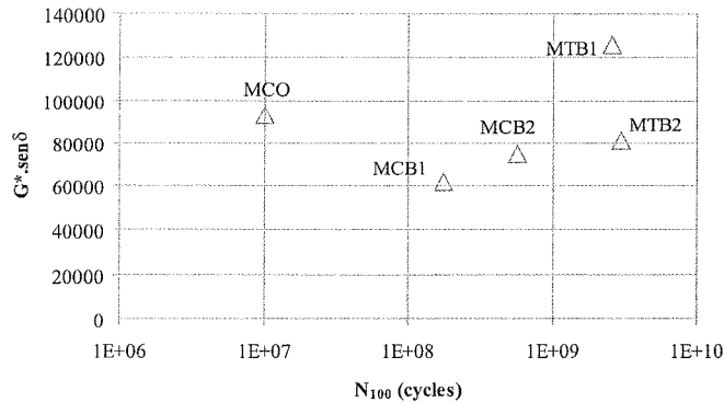
Figure 14. Fatigue life versus G^* \cdot \sin \delta
