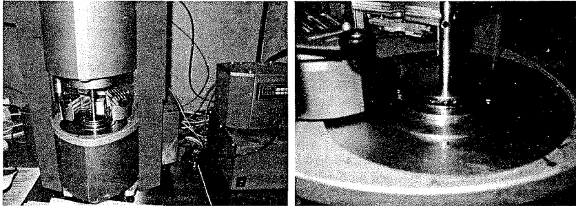
Figure 6. Rheometer and parallel plates
