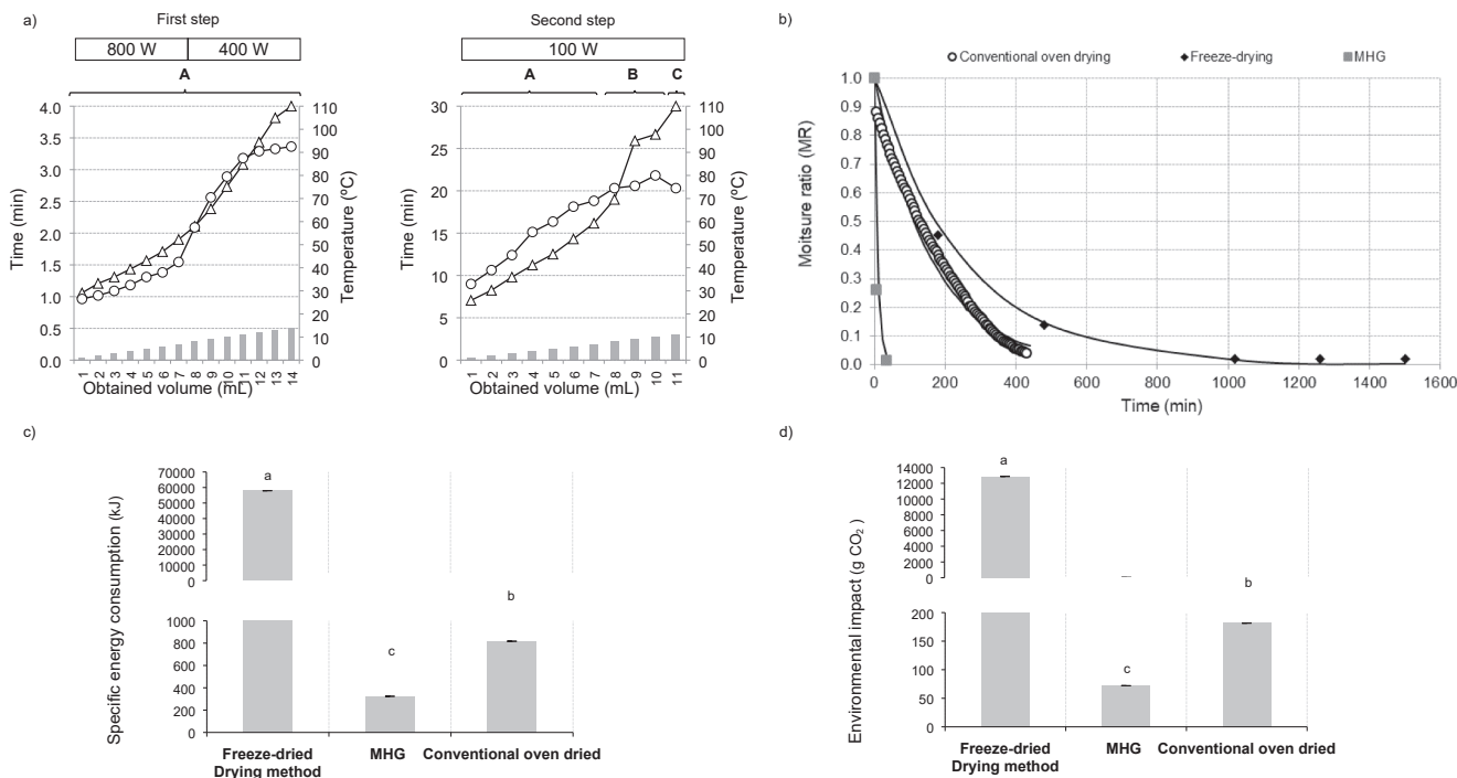
Fig. 2. a) Extraction kinetics of discontinuous optimized MHG treatment from C. crispus by the combination of different irradiation powers: first step (800 and 400 W for 2 min, respectively) and second step (100 W for 30 min). Symbols: Extraction time (triangles), vessel temperature (circles) and collected volume (bars). Typical phases of MHG treatment: heating phase (A), extracting phase (B) and burning phase (C). b) Drying kinetic of C. crispus seaweed by tested dried methodologies. Symbols: line (Page model). Note here that freeze-drying data (x-axis) were shortened (around 14,200 min) in order to improve data visualization. c) Estimated specific energy consumption of different drying procedures from C. crispus macroalgae. Data are given as mean \pm standard deviation. Data values with different superscript letters are statically different ( p \leq 0.05 ). d) Derived environmental impact. Data are given as mean \pm standard deviation. Data values with different superscript letters are statically different ( p \leq 0.05 ).
