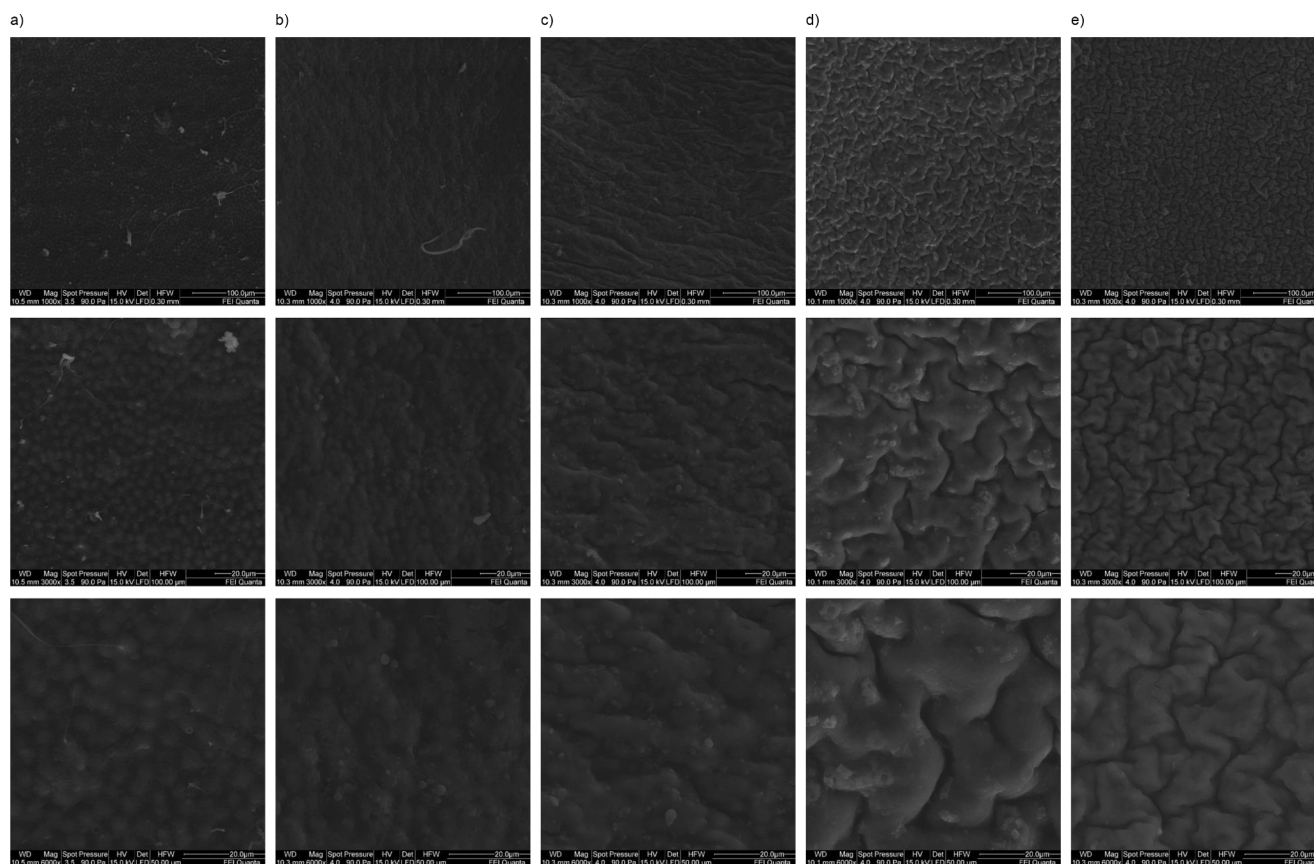
Fig. 3. Microscopic structure images of C. crispus samples untreated (a), defrosted macroalgae (b) and dried red seaweed (freeze-dried (c), MHG (d) and conventional oven dried (e)). Upper, middle and lower images with magnification of x1000, x3000 and x6000, respectively.
