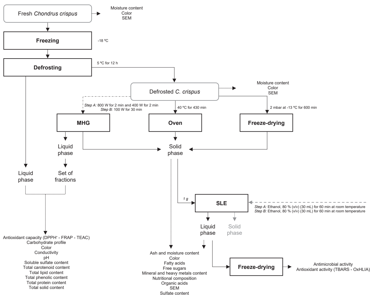
Fig. 1. Flowchart of studied dehydration processes of edible Chondrus crispus red seaweed. DPPH • : 1,1-Diphenyl-2-picryl-hydrazyl; FRAP: Ferric reducing antioxidant power; MHG: Microwave hydrodiffusion and gravity; OxHLIA: Oxidative haemolysis inhibition; SEM: Scanning electron microscopy; SLE: Solid-liquid extraction; TBARS: Thiobarbituric acid reactive substances; TEAC: Trolox equivalent antioxidant capacity.
