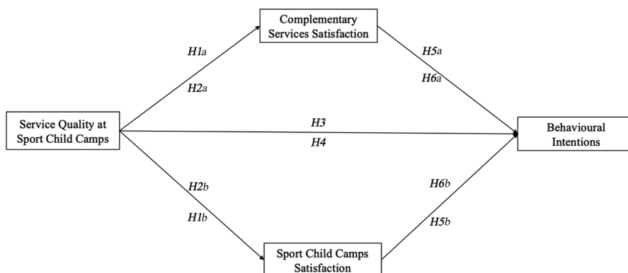
Figure 1. Hypothesized model
