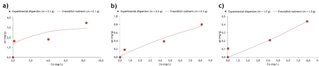
Figure 5 - Sorption isotherms for the Freundlich model with Cu and soil masses of 0.1 g (a), 0.5 (b) and 1.0 g (c)
