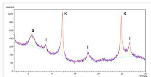
Figure 3 - X-ray diffraction of the soil sample (< 2 μm)
