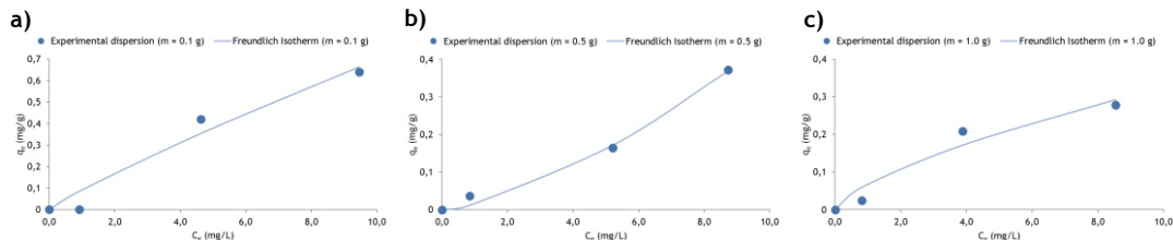
Figure 4 - Sorption isotherms for the Freundlich model with Cr and soil masses of 0.1 g (a), 0.5 (b) and 1.0 g (c)
