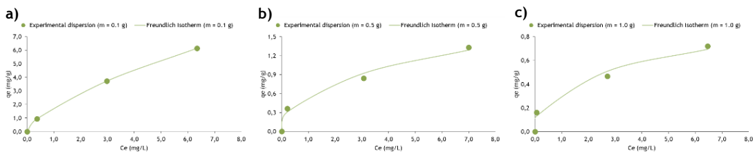
Figure 6 - Sorption isotherms for the Freundlich model with Zn and soil masses of 0.1 g (a), 0.5 (b) and 1.0 g (c)
