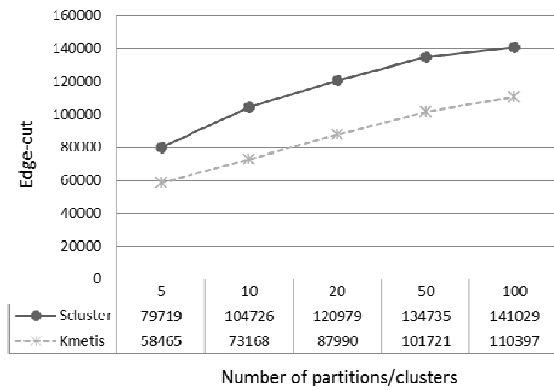
Graph: dblp-2010
