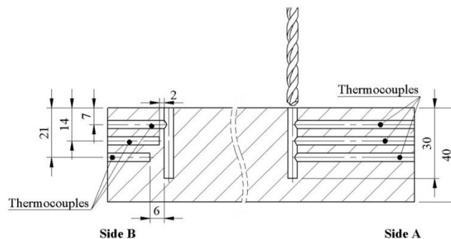
Fig. 2 - Illustration of the thermocouples positions
