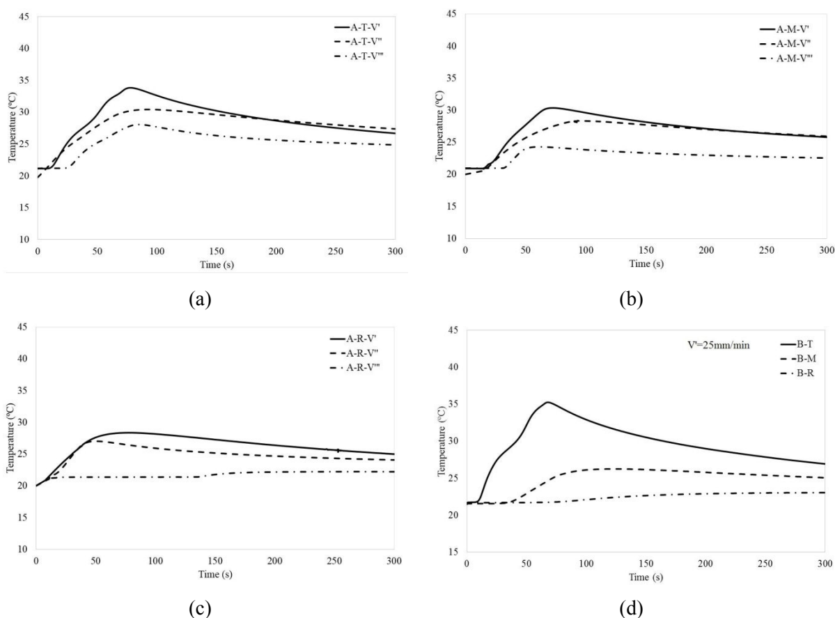
Fig. 6 - Evaluation of temperature at different feed rates and positions of thermocouples
