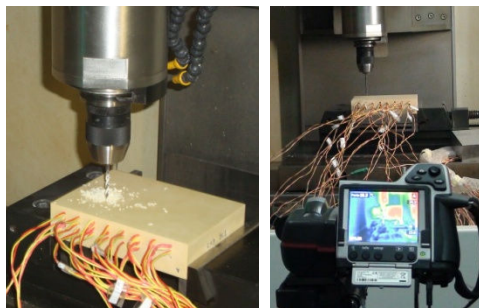
Fig. 3 - Drilling process of composite materials
