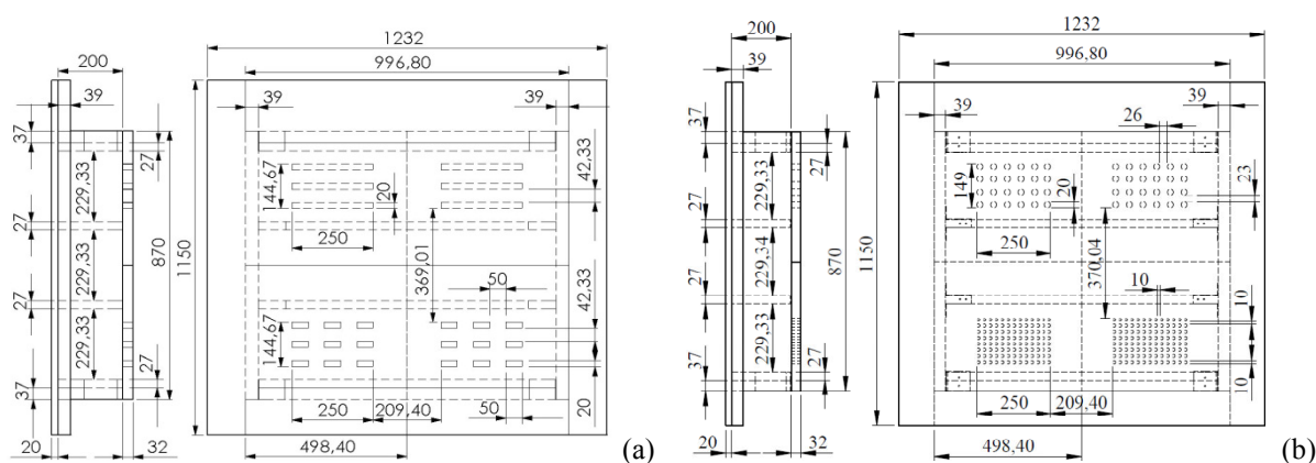
Fig. 2 - Geometry of wooden slabs: a) slab_1_2 rectangular perforations, b) slab_3_4 circular perforations.
