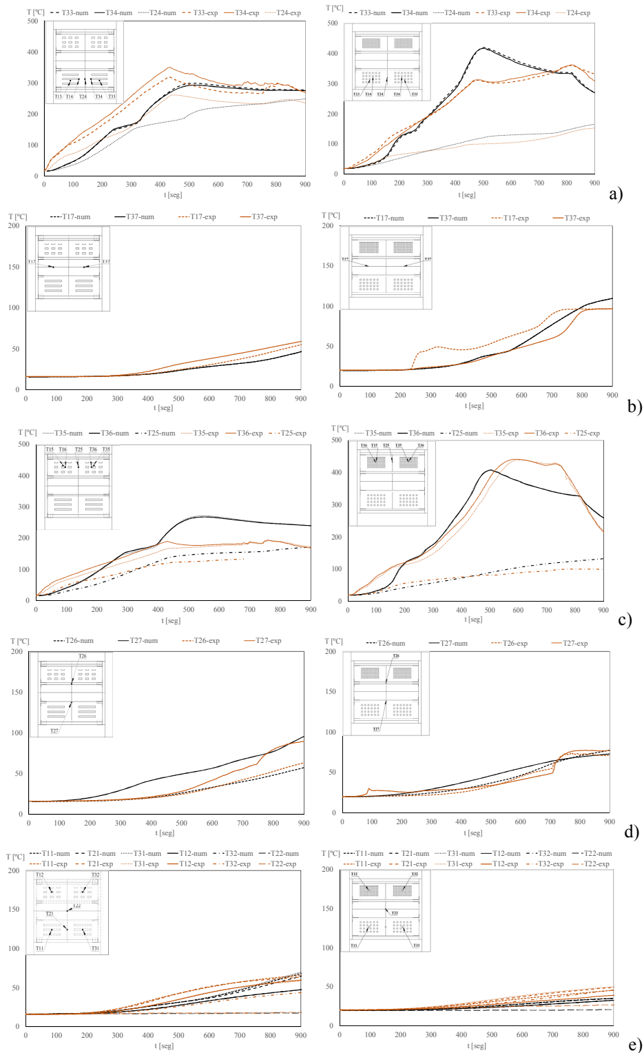
Fig. 9 - Time-temperature history for each wooden slab (slab_1_2 and slab_3_4): a) on cell 3, b) on cell 2, c) on cell 1, d) on beams, e) at unexposed surface.
