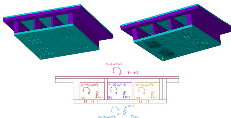
Fig. 7 - Numerical model for each wooden slab.
