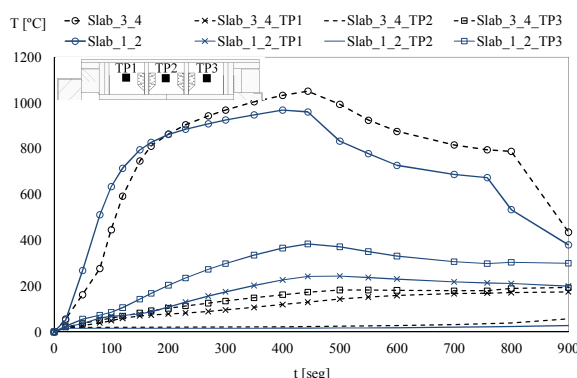
Fig. 8 - Heating curves.
