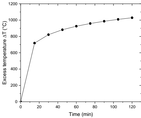
FIGURE 2. T-time curve according to ISO834
