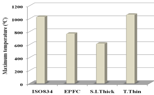
FIGURE 5.2. Maximum gas temperature (various formulations)
