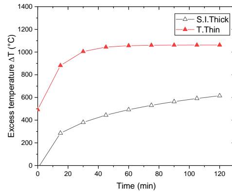
FIGURE 4. Temperature evolution (Swedish standard) for two limiting assumptions
