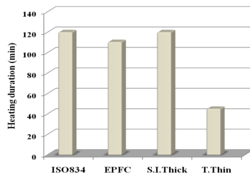
FIGURE 5.1. Heating phase duration (various formulations)
