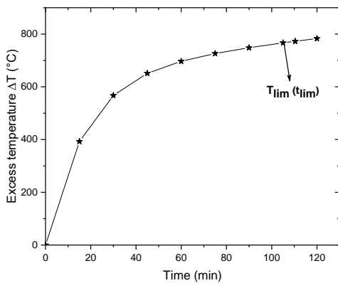
FIGURE 3. The EPF curve of gas temperature
