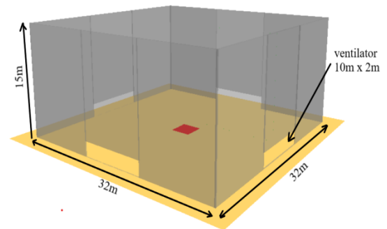
FIGURE 1. Sketch of the compartment geometry
