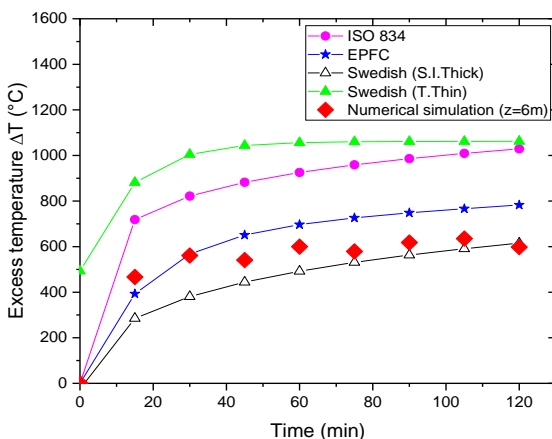
FIGURE 6. Temperature histories (All formulations)
