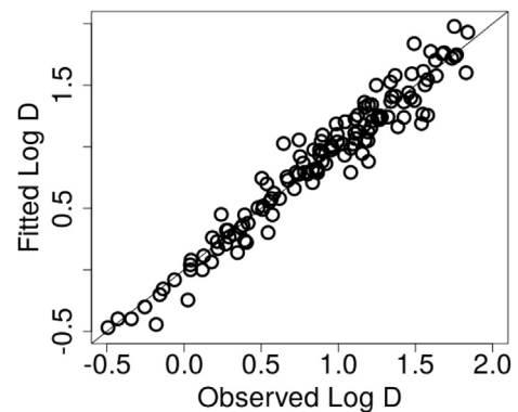
Fig. 4. Relationship between the observed \log D extracted from the primary studies and the \log D fitted by the meta-analytical mixed-effects linear model.
