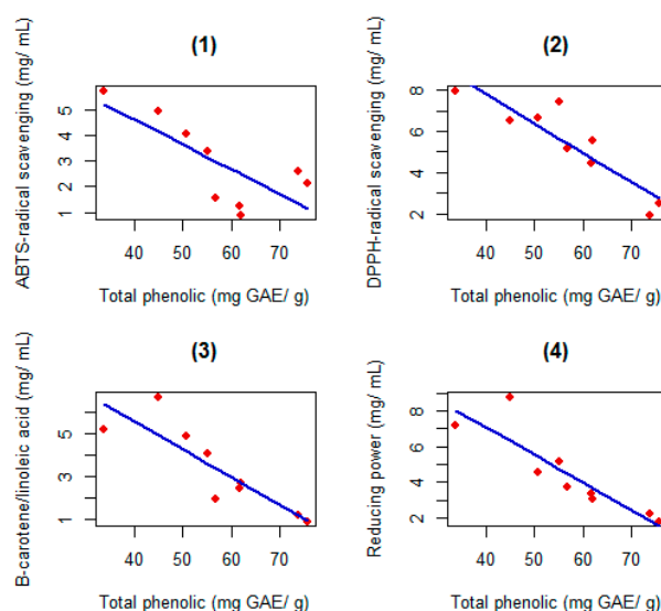
Figure 1. Regression equations estimated for the four evaluation methods of the antioxidant activity in relation to the amounts of total phenols. (1) y = -0.0965x + 8.4587 ( R^2 = 57\% , p < 0.01 ); (2) y = -0.1429x + 13.5332 ( R^2 = 82\% , p < 0.01 ); (3) y = -0.1294x + 10.7458 ( R^2 = 76\% , p < 0.01 ); (4) y = -0.1539x + 13.2256 ( R^2 = 79\% , p < 0.01 ).
