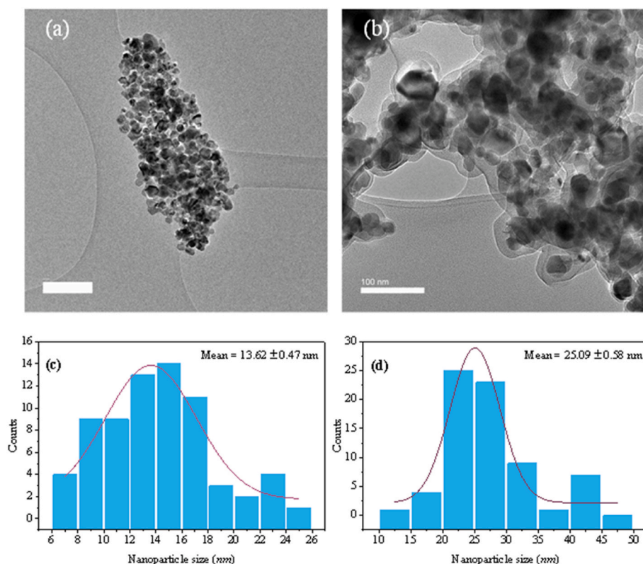
Fig. 3. TEM images of (a) NiFe and (b) NiFe@C-PF127 MMCSNPs. Nanoparticles size distribution calculated with ImageJ for (c) NiFe and (d) NiFe@C-PF127. 37.
