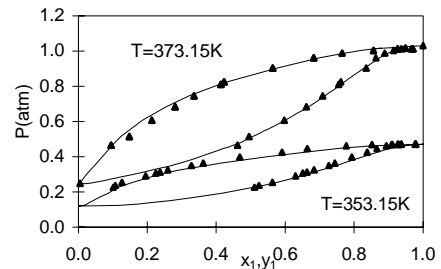
Fig. 7. VLE of H 2 O (1) + propanoic acid (2): \blacktriangle Exp. (Gmehling and Onken, 1977a, pgs.222 and 224); — GCA-EOS.
