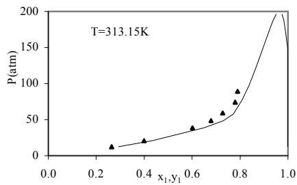
Fig. 3. VLE of ethane (1) + oleic acid (2): \blacktriangle Exp. (Peter et al. , 1991); — GCA-EOS.
