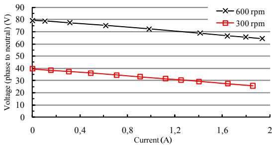
Fig. 12: Phase to neutral voltage versus current.
