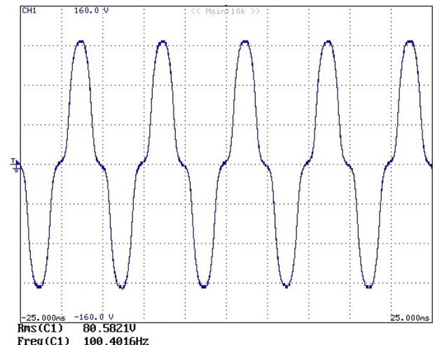
Fig. 10: No load phase to neutral voltage at 600 rpm (voltage scale: 40 V/div; time scale: 5 ms/div).
