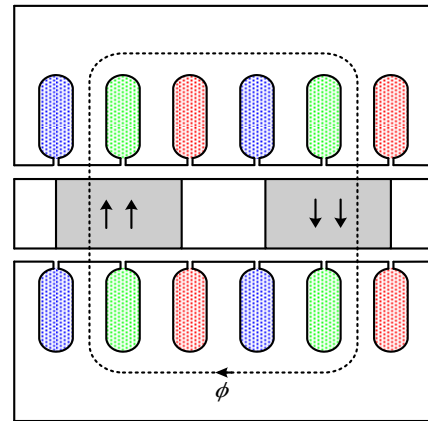
Fig. 3. 2D plane of the axial flux permanent magnet machine.
