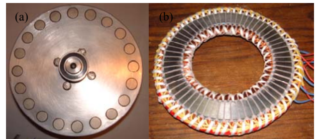
Fig. 9: Generator rotor disk (a) and one stator ring (b).
