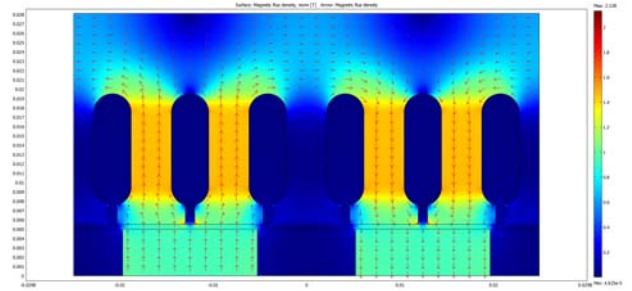
Fig. 5. Magnet flux density at the middle plane, under no load condition.
