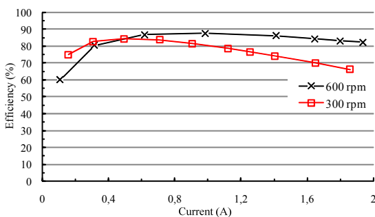
Fig. 14: Efficiency versus current.
