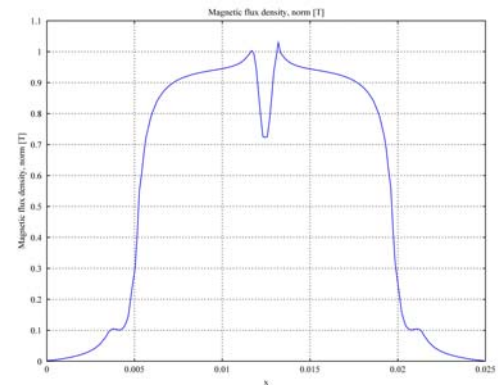
Fig. 6. Air gap flux density under no load condition.
