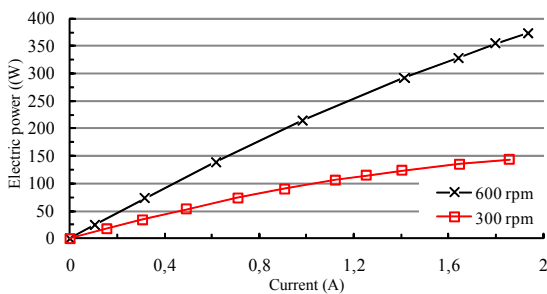
Fig. 13: Electric power versus current.
