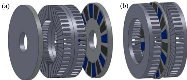
Fig. 2. Double sided axial flux machine structures. (a) internal stator. (b) internal rotor.
