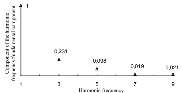
Fig. 11: Harmonic components in no load phase to neutral voltage.
