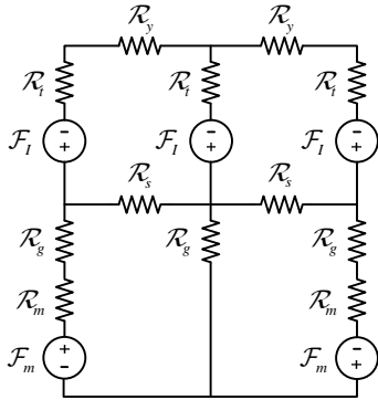
Fig. 4. Reluctance network over one pole pitch.
