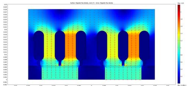
Fig. 7. Magnet flux density at the middle plane, under load condition.
