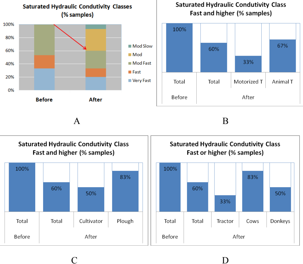
Figure 4: Effects of treatments on Saturated Hydraulic Conductivity class distribution at surface soil layer (0-0.05 m depth): A – Operations global effect; B – Motorized and Animal Traction effects; C – Implement effect; D – Traction mean effect
