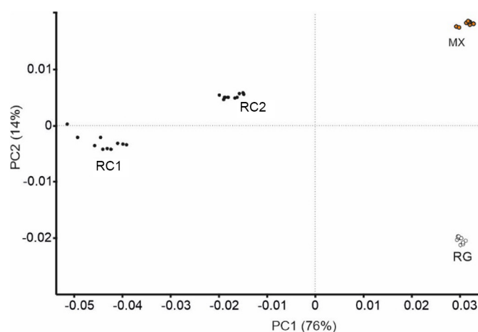
Figure 9. Principal component analysis score plot corresponding to the classification of raw cow milk, raw goat milk, and the mixture of cow and goat milks.
