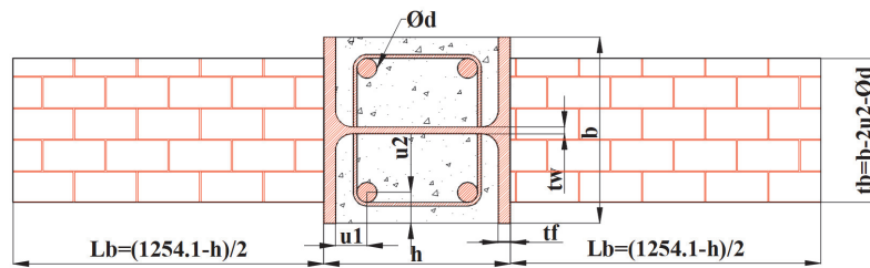
Figure 1: Partially encased column embedded on wall.
