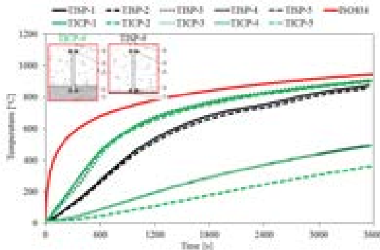
Fig. 19 - Temperature evolution in model's TISP and TICP, submitted to fire scenario 2.
