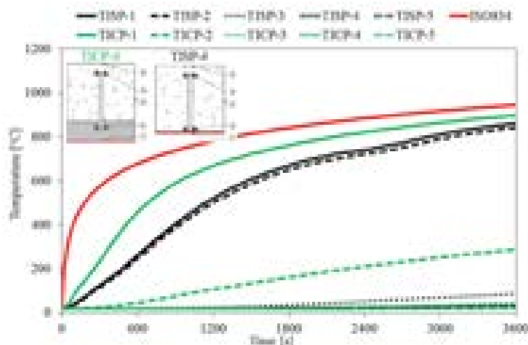
Fig. 17 - Temperature evolution in model's TISP and TICP, submitted to fire scenario 1.
