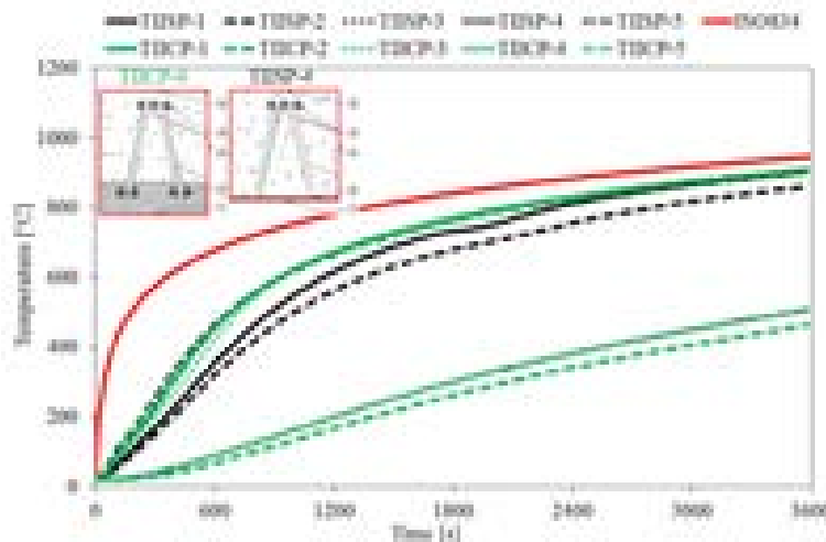
Fig. 20 - Temperature evolution in model's TIISP and TIICP, submitted to fire scenario 1.
