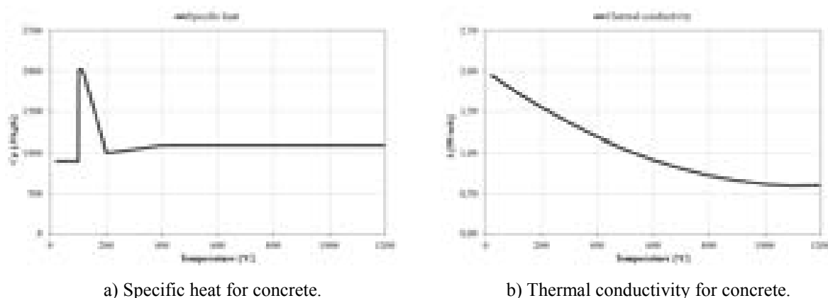
Fig. 4 - Thermal properties of concrete.
