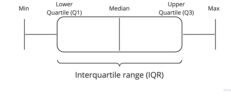
Figure 4.3: BoxPlot.
