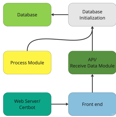
Figure 5.1: Containers dependency.
