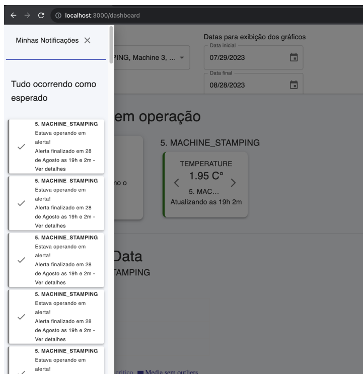
Figure 6.4: Notification drawer.
