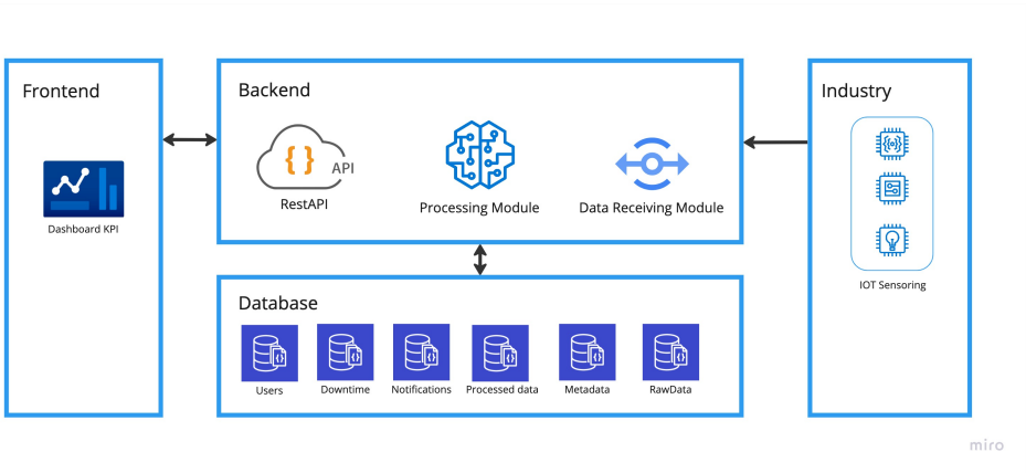
Figure 4.1: System architecture.
