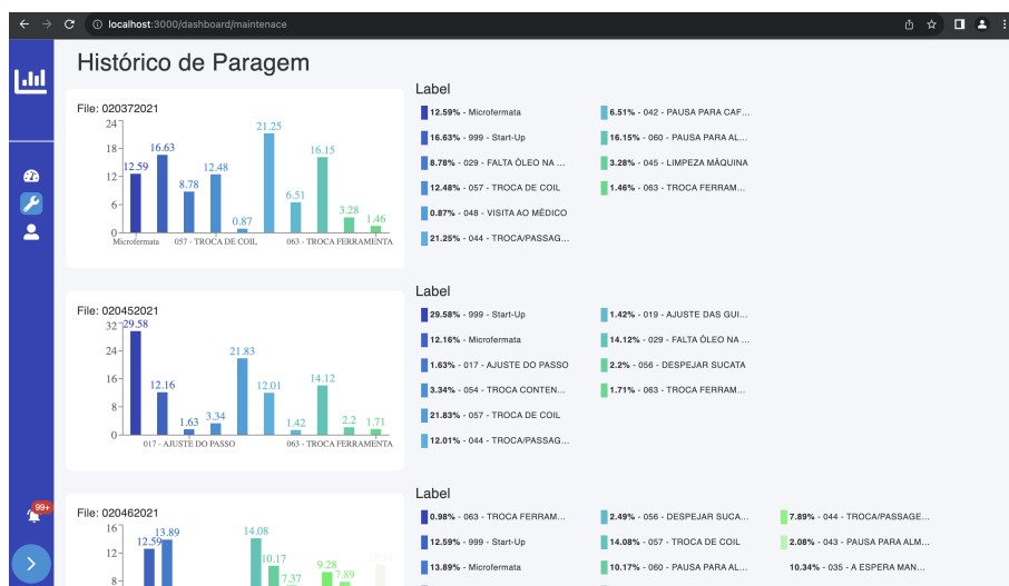
Figure 6.7: Downtime graph.
