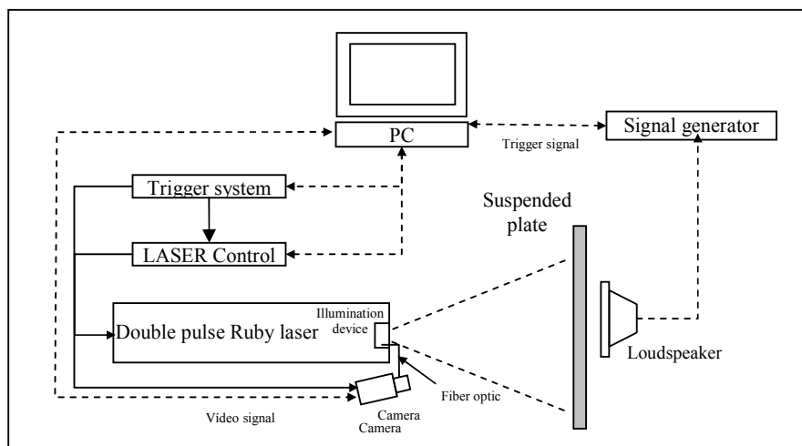
Figure 1- Schematic presentation of the experimental set-up.
