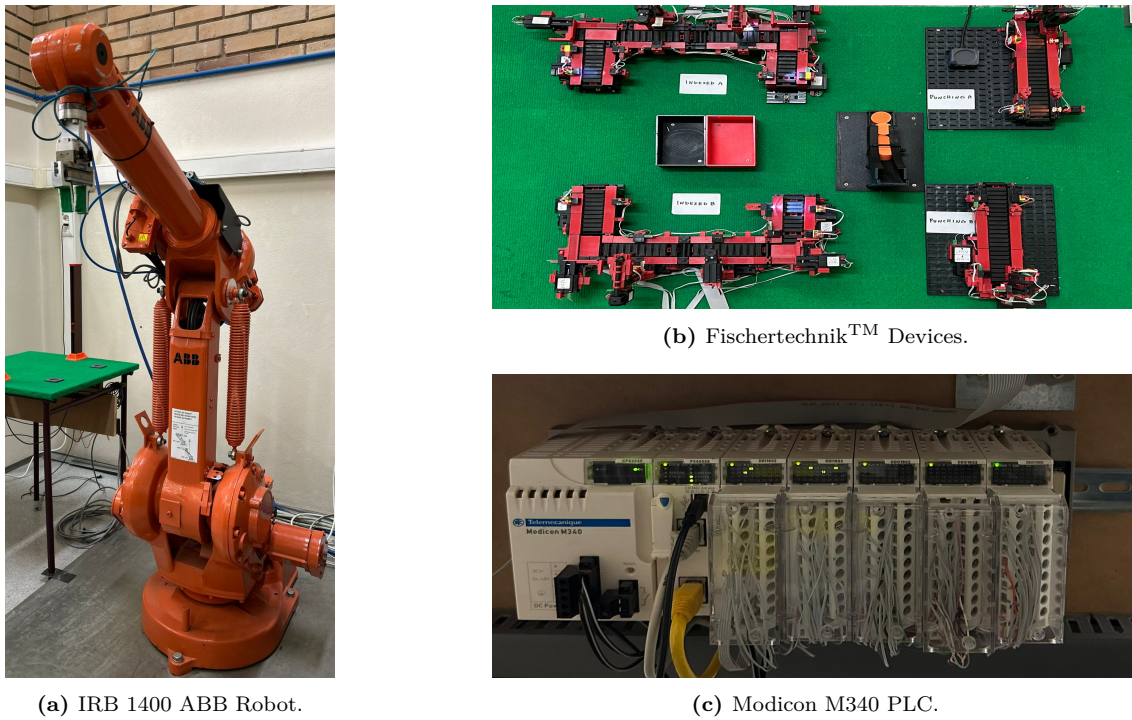
Figure 4.1: Small-Scale Production Experimental Layout.
