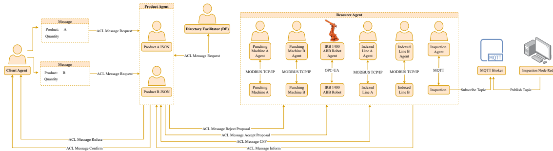
Figure 4.4: Small-Scale Production System Diagram.
