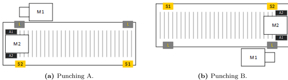
Figure 4.2: Technologically Layout of Punching Machine.
