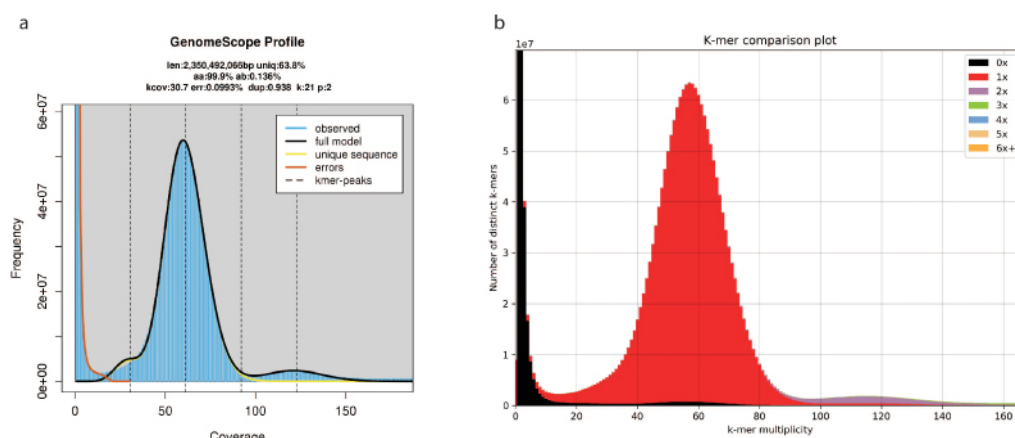
Figure 3. (a) GenomeScope2 k-mer 0 distribution displaying the estimation of the genome size (len), the homozygosity (aa), the heterozygosity (ab), the mean coverage of k-mer for heterozygous bases (kcov), the read error rate (err), the average rate of read duplications (dup), the size of the k-mer used on the run (k), the ploidy (p), and percentage of the genome that is unique (not repetitive) (uniq). (b) M. margaritifera genome assembly assessment using the KAT comp tool to compare the Illumina paired-end k-mer content within the genome assembly. Different colours represent the read k-mer frequency in the assembly.
