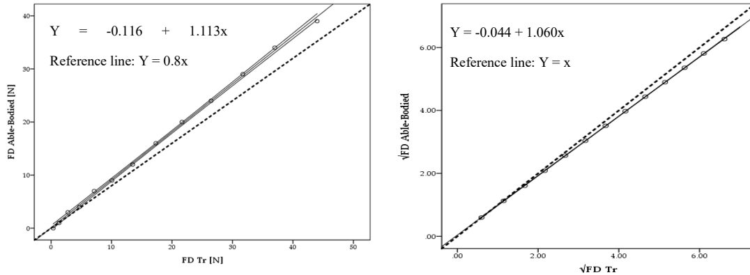
Figure 2. Scattergram, CI lines, tendency line (black) and reference line (dashed black) between able-bodied and Tr model for absolute drag (FD) values (left) and after square root ( \sqrt{\phantom{x}} ) transformation (right).
