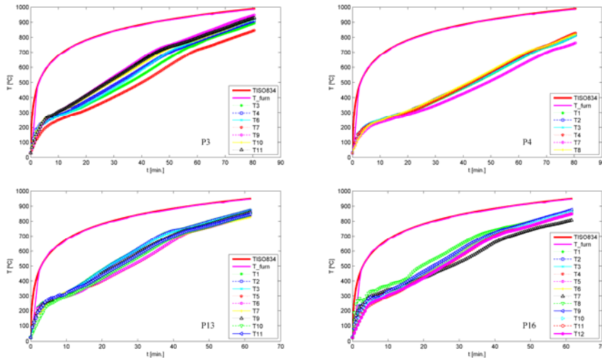
Figure 10 - Temperature evolution results of intumescent protected solid and cellular beams.
