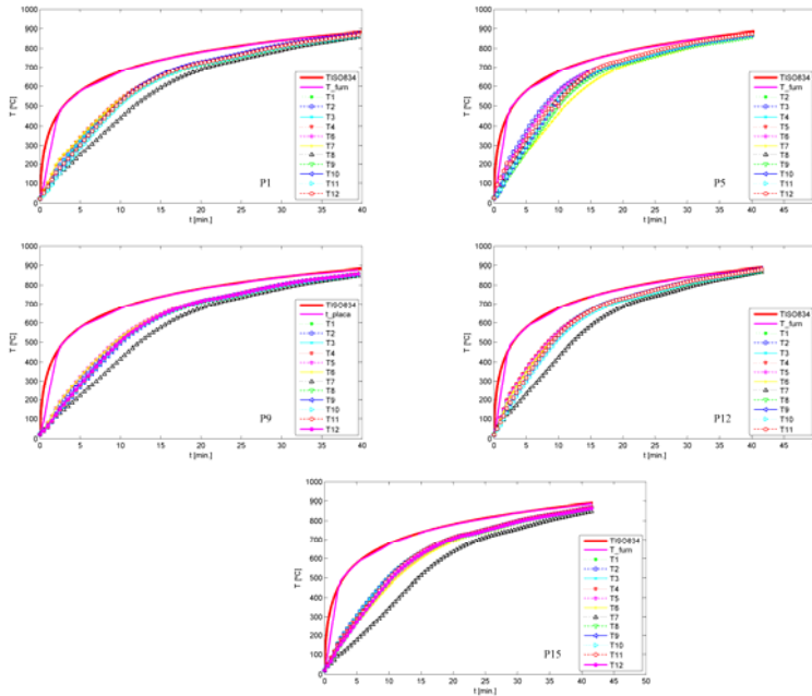
Figure 8 - Temperature evolution results of unprotected solid and cellular beams.
