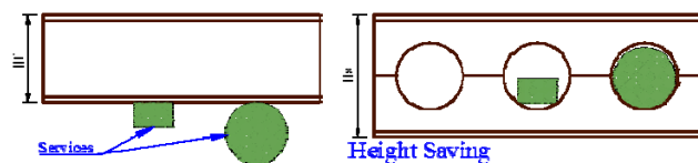
Figure 1 – Ceiling height saving from CB installation.
