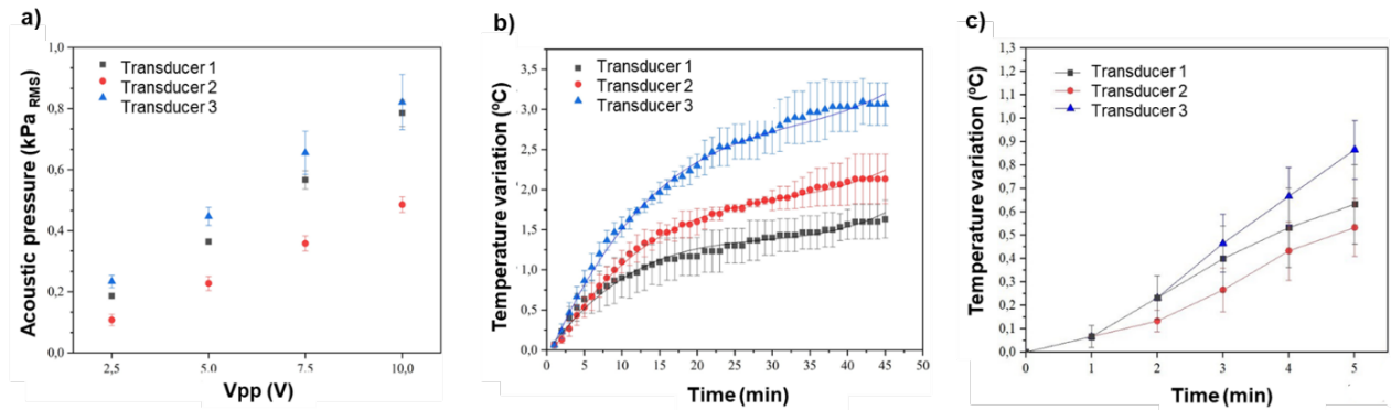
Figure 1 - a) Pressure measured in the culture well, as a function of the voltage; b) Temperature variation in the culture well, when a sinusoidal electrical signal of 10 V_{pp} is applied; c) inset of temperature variation for 5 min.
