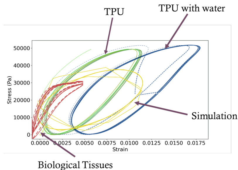
Figure 7 - Hysteretic behaviour of the experimental results compared with the simulation.
