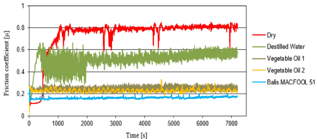
Figure 2 - The comparative wear analysis or friction coefficient results between OMWW and conventional cutting fluids.
