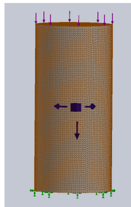
Figure 3 - Generated mesh.
