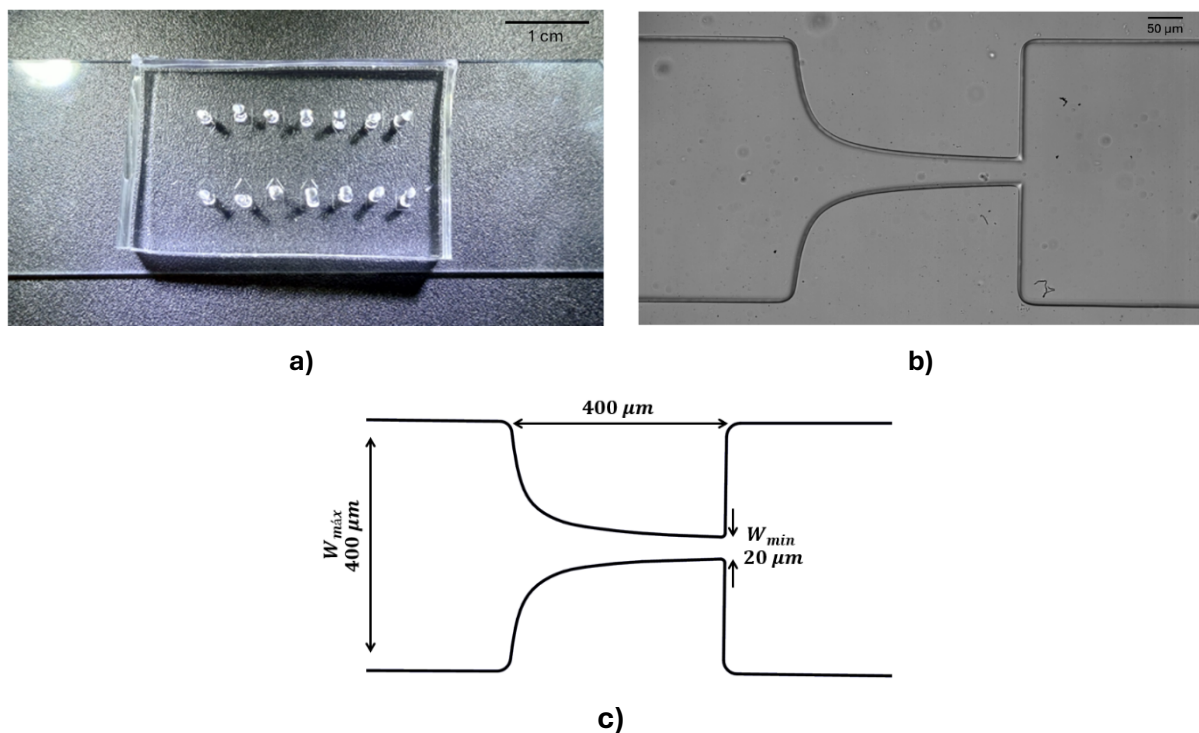
Figure 3 - a) PDMS mould of the microfluidic channels in set of 7, where the inlets and outlets punch holes are visible; b) Microscope image (obj. 20×) of the hyperbolic contraction of the PDMS microchannel; c) Geometry and main dimensions of the microchannel
