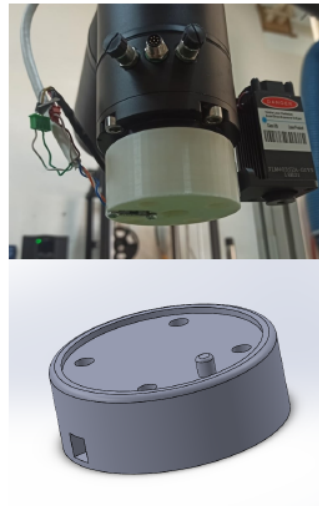
(c) Attachment for laser engraver.
