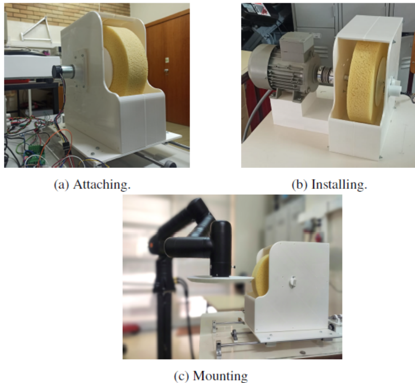
Figure 1 - Step-by-step assembly stages of the manipulator robot.
