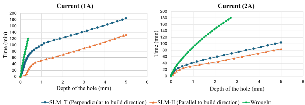
Figure 1 - Time machining vs depth of the hole.
