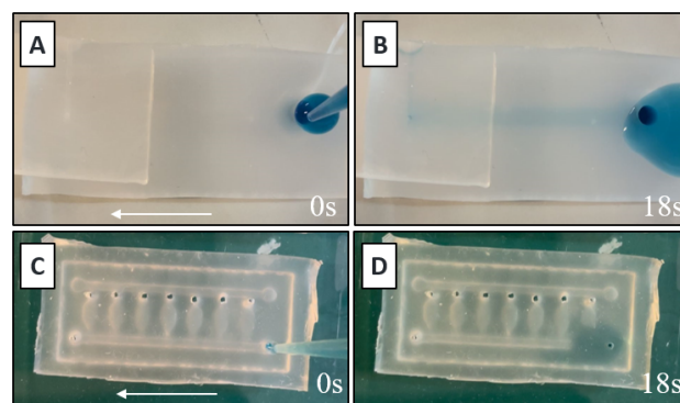
Figure 4 - Devices modified with 2.5% PEO: (A) Device I at 0s and (B) after 18s. (C) Device II at 0s and (D) at 18s.
