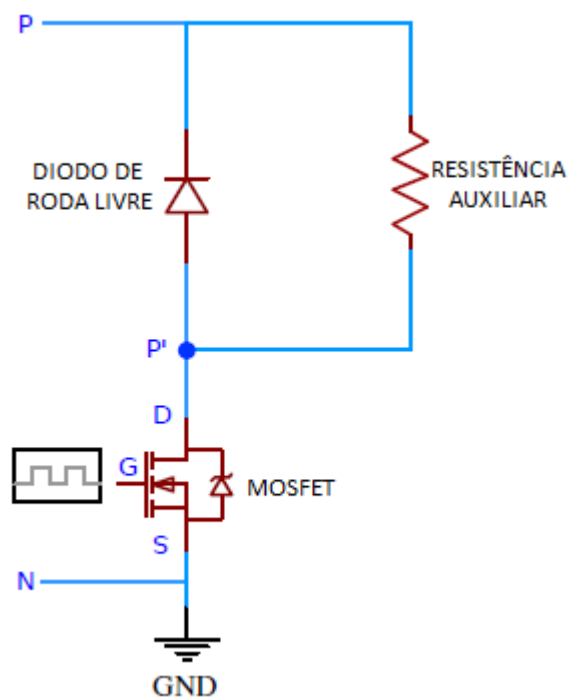
Figura 31 – Conversor Buck .
