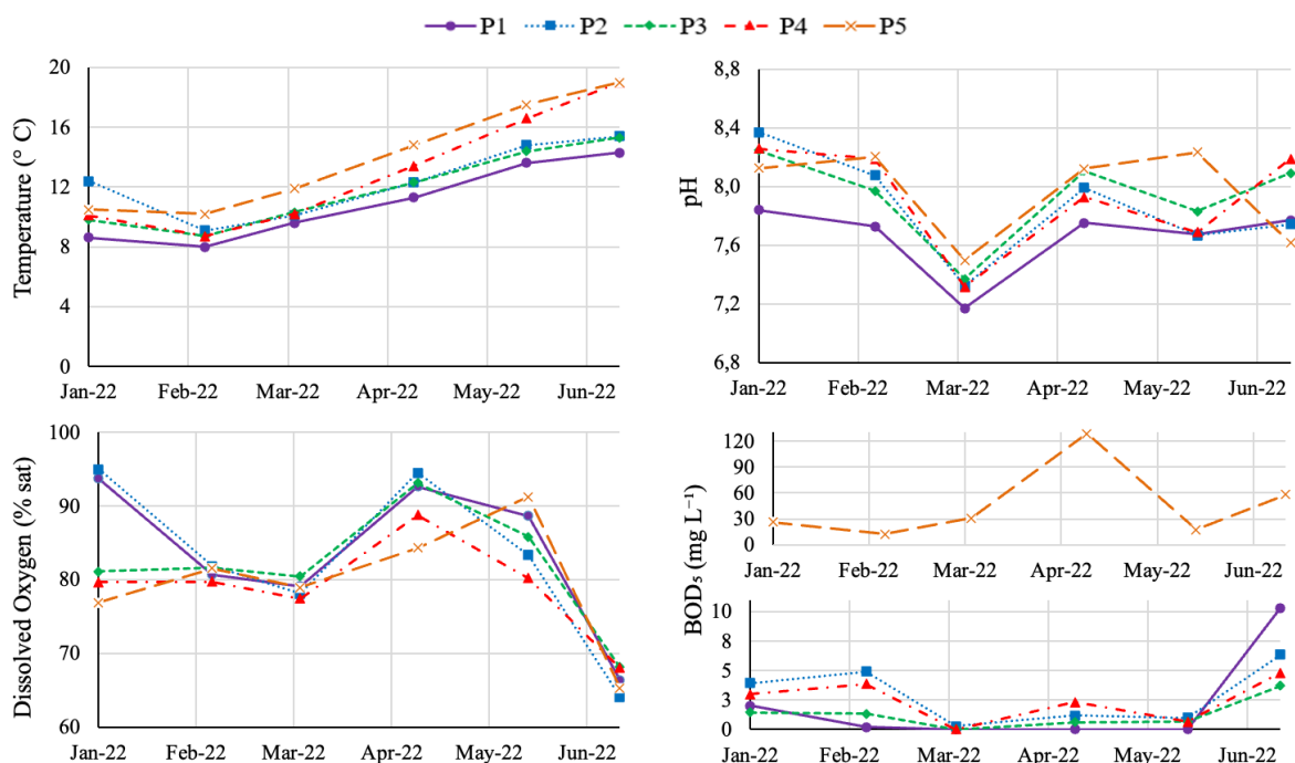
Fig. 2. Water quality parameters (temperature, pH, dissolved oxygen, and BOD 5 ) of the Fervença river (January – June 2022)
