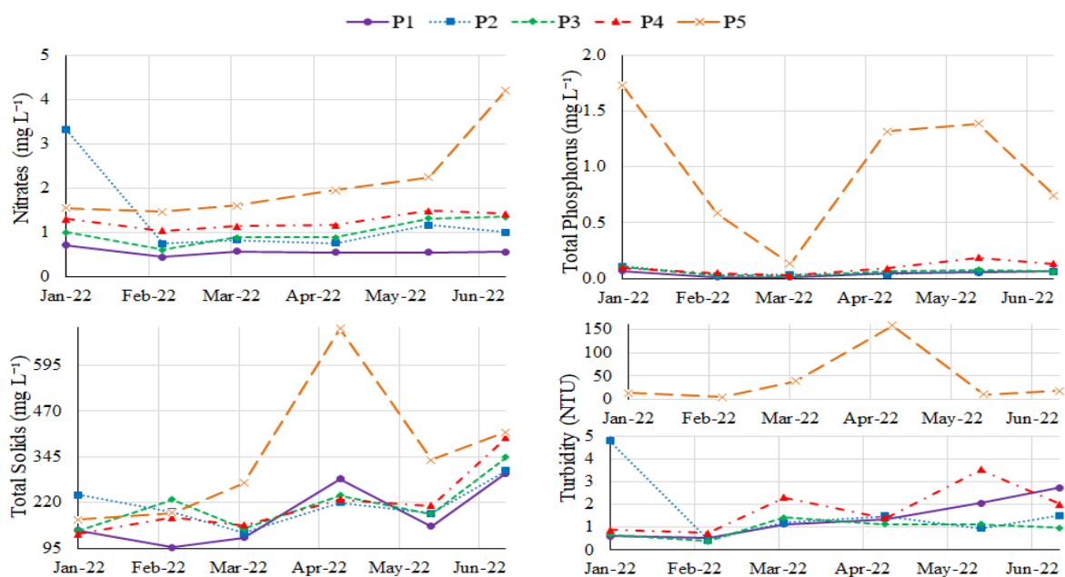
Fig. 3. Water quality parameters (nitrate, total phosphorus, total solids, and turbidity) of the Fervença river (January – June 2022)
