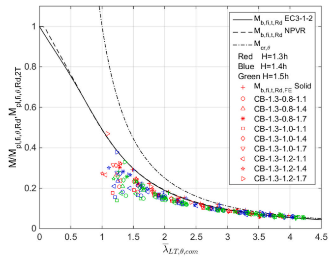
(b) Distributed load, \theta=500^{\circ}\text{C}
