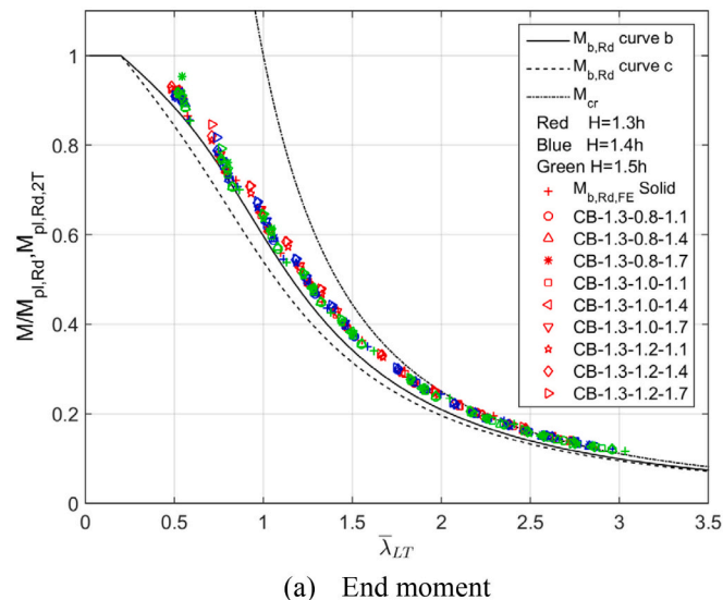
Fig. 7. Comparison between numerical normalized collapse moments and LTB analytical reduction factors versus non-dimensional slenderness at \theta = 20 °C.
