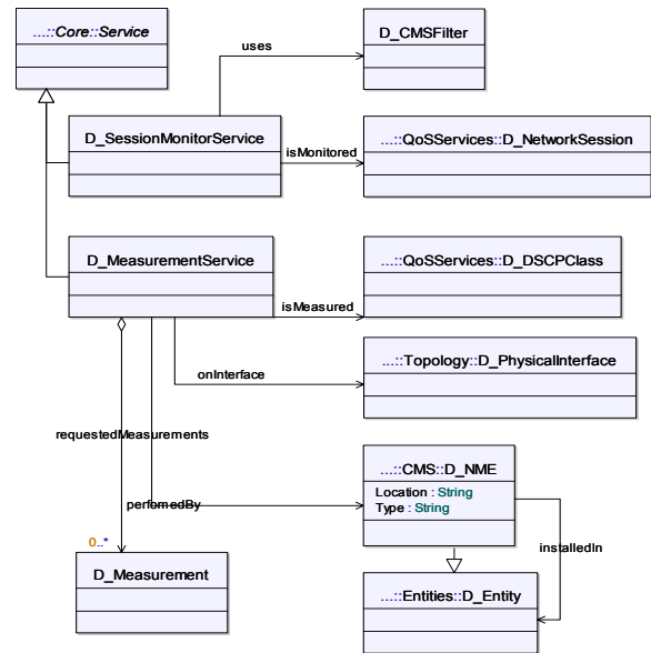
Fig. 7 - The main class diagram of CMSServices package.
