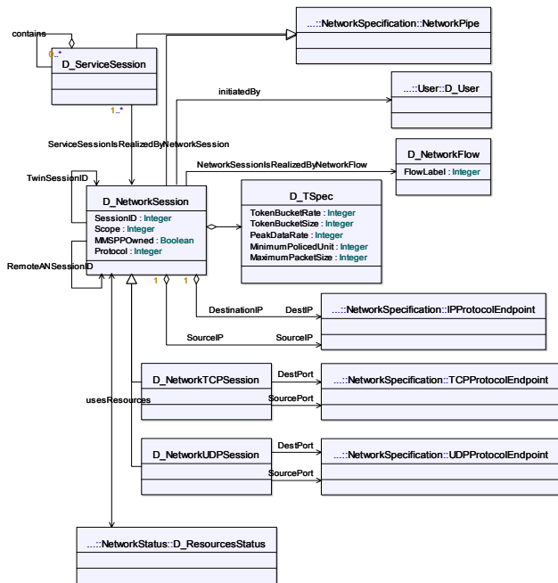
Fig. 6 - The main class diagram of QoSServices package.
