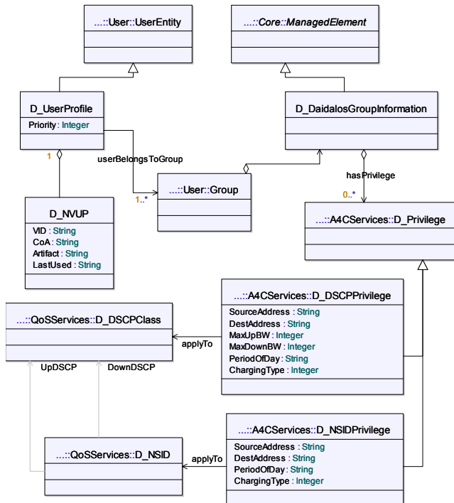
Fig. 4 - The main class diagram of User package.
