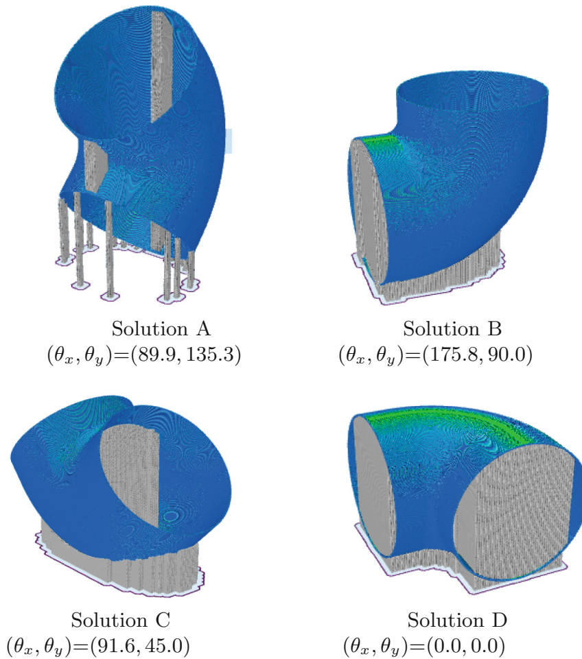
Fig. 11. Representation of the solutions A, B, C and D of 45 Degree Short model.
