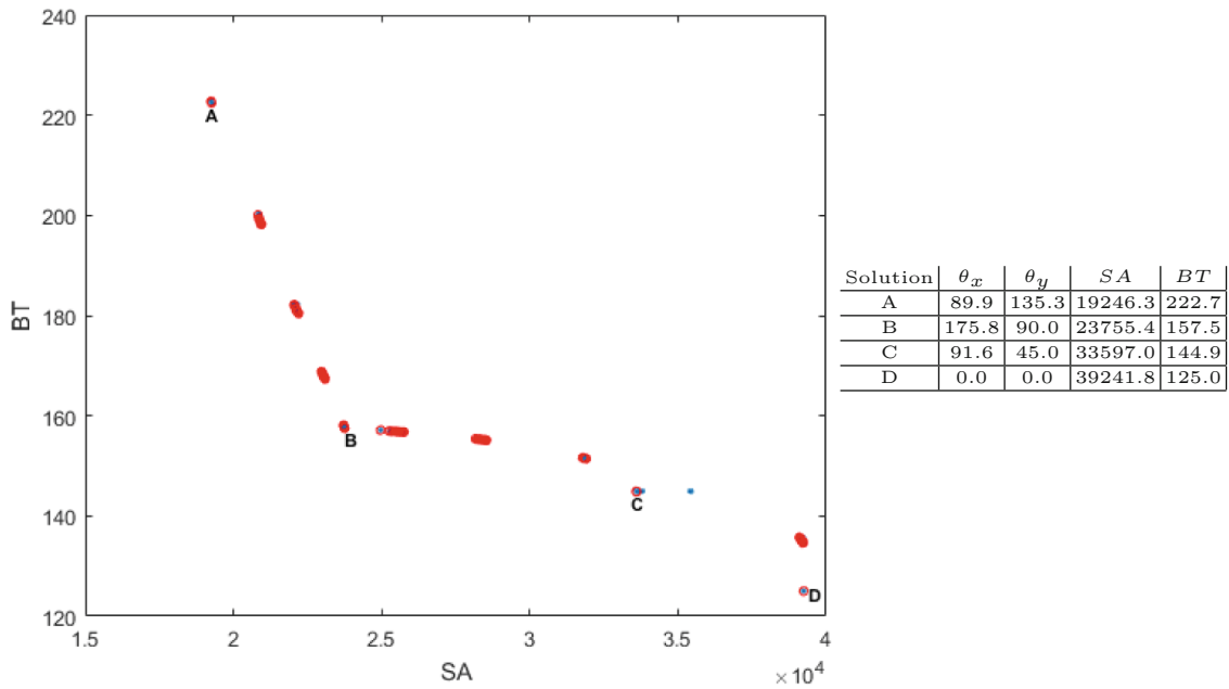
Fig. 10. Pareto front and representative solutions for the 45 Degree Short model.
