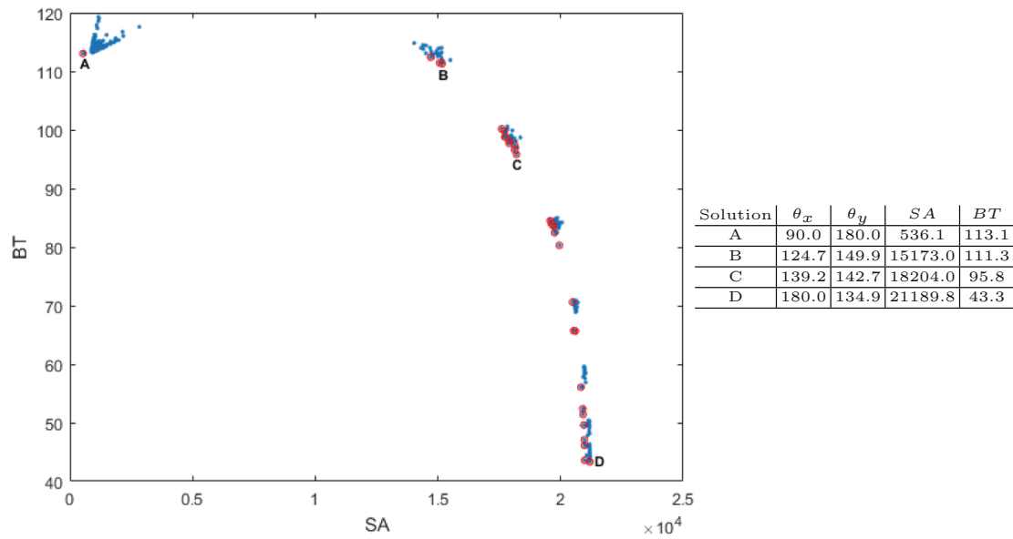
Fig. 4. Pareto front and representative solutions for the Rear Panel Fixed model.
