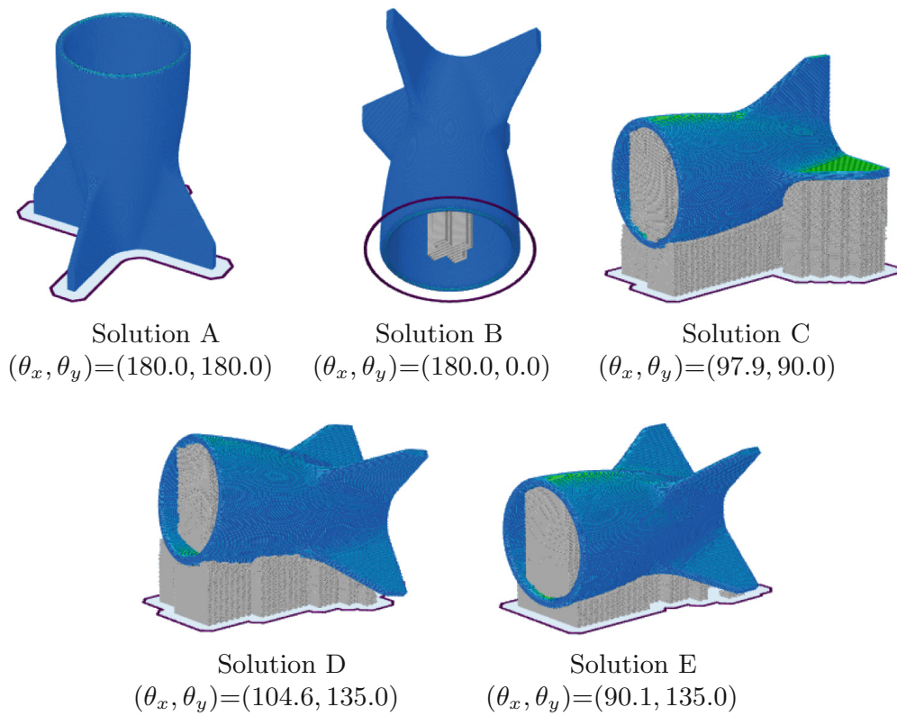
Fig. 9. Representation of the solutions A, B, C, D and E of Rocket Shot model.
