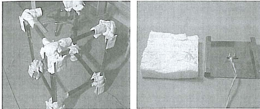
a) Relative position for plate thermocouples.
