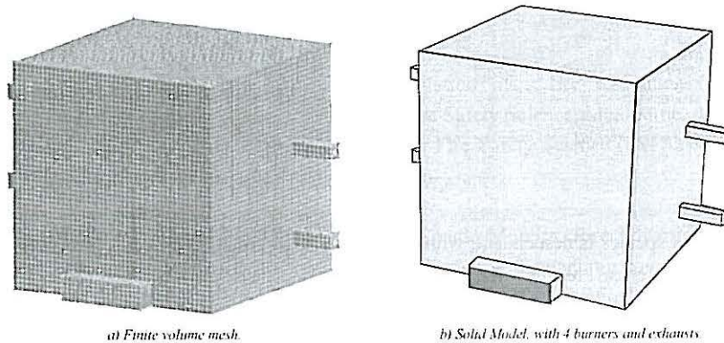
Fig. 5. Model for fire-resistance furnace.
