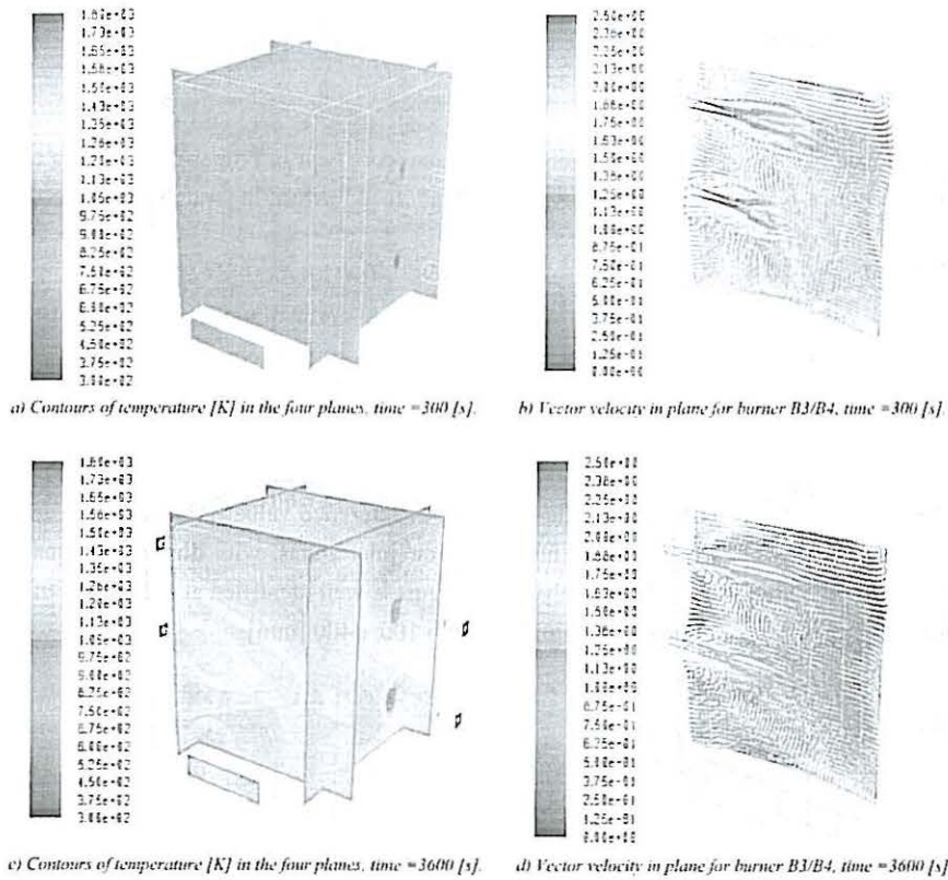
Fig. 6. Numerical results for Test 1.
