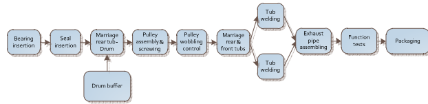
Fig. 1. Layout of the production line case study.
