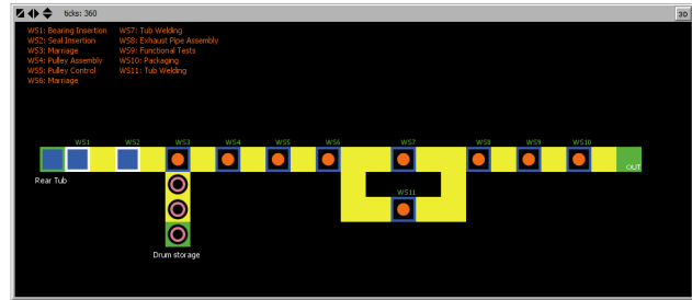
Fig. 4. Test scenario with the WS7 having an increased processing time
