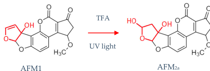
Figure 4. Reaction of AFM1 with trifluoroacetic acid (TFA) and UV light.
