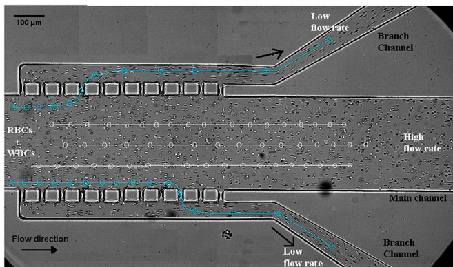
Fig. 5. Microscope image (20 \times objective) at zone A (see Fig. 1) of the micro-device. The lines with symbols represent schematically expected trajectories of different blood cells flowing through the main and branch microchannels.
