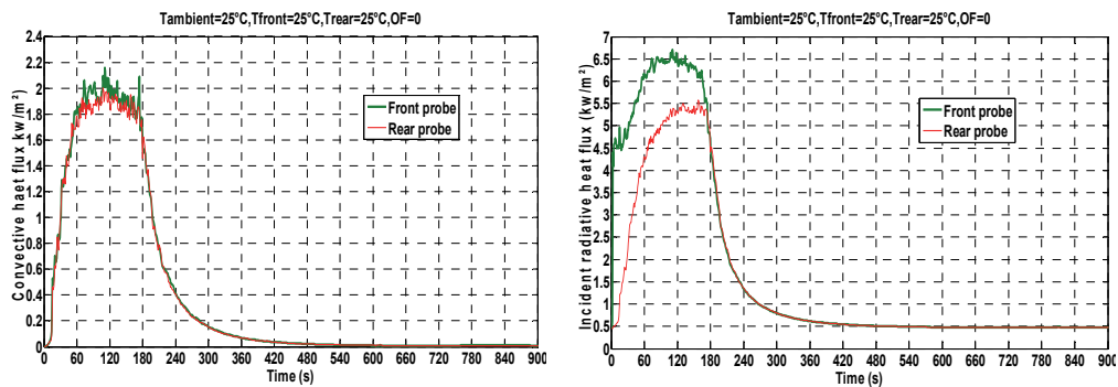
Figure 1: Convective (left) and radiative heat flux evolution in a fully confined case.
