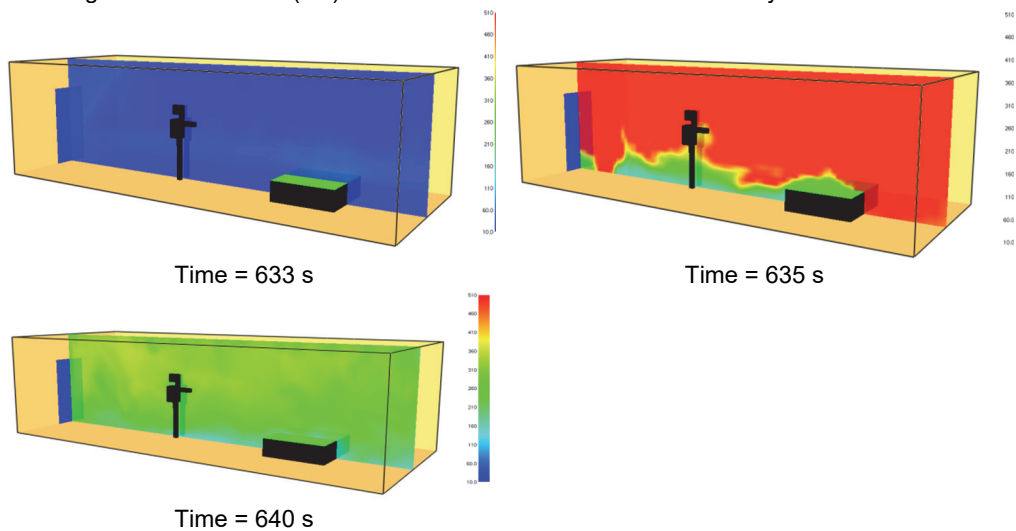
Figure 2: Temperature evolution in a ventilation-induced (MV) flashover.
