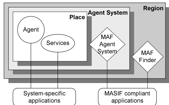
Figure 2 - MASIF architecture.
