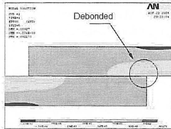
Figure 2 – Numerical simulation of a single lap joint with an unbonded region.
