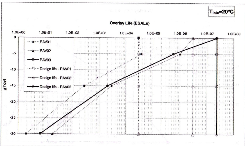
Figure 10. Overlay life as function as \Delta T_{ovl} , for traffic + temperature loading for uniform temperature drop in bituminous layers
