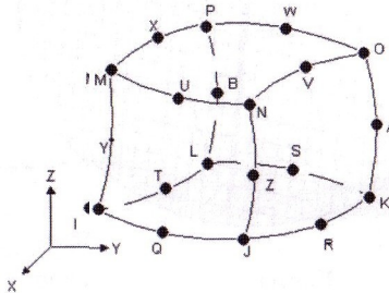
Figure 4. 3-D twenty-node structural solid element
