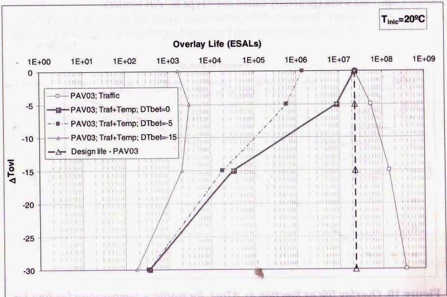
Figure 9. Overlay life as function as \Delta T_{ovl} , for traffic loading only and for traffic loading + temperature loading – T_{inc}=20^{\circ}C
