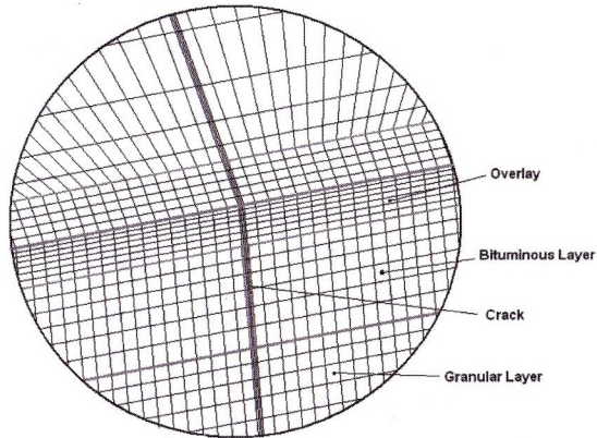
Figure 2. Crack location
