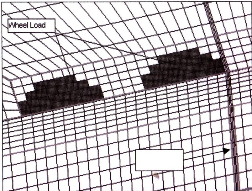
Figure 3. Wheel load configuration
