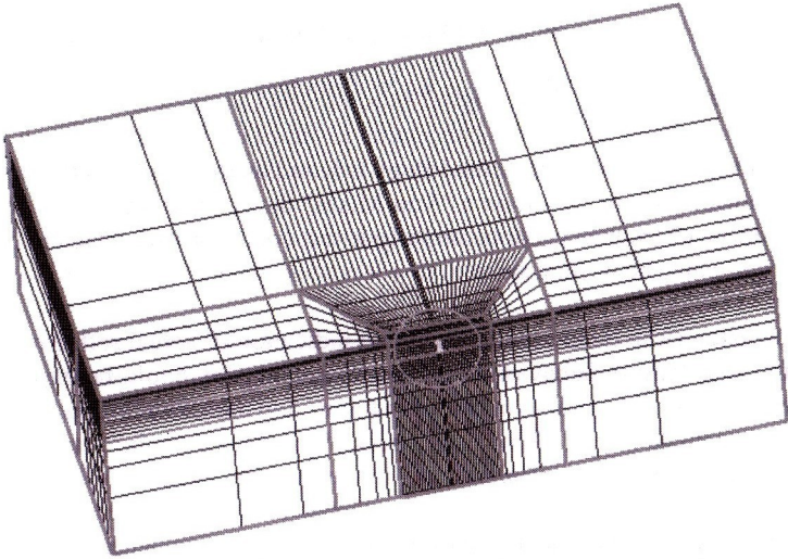
Figure 1. 3D Representation of Finite Element Mesh
