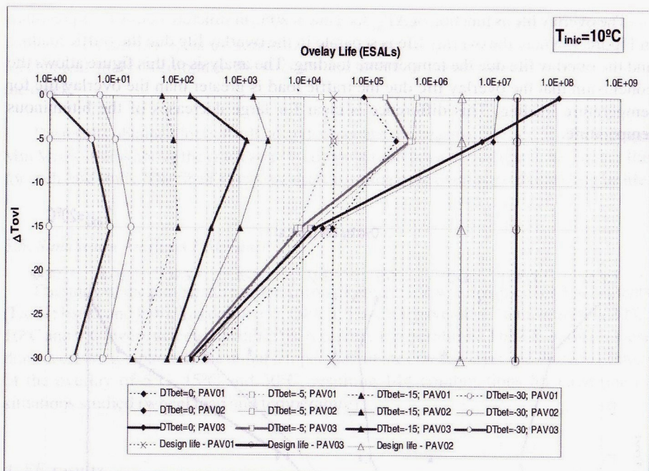
Figure 6. Overlay life as function as \Delta T_{ovl} , for initial temperature of 10^{\circ}\text{C}
