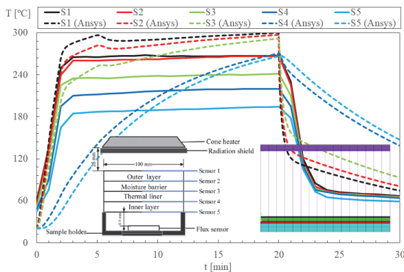
a) Comparison of the numerical results with the experimental results of M. Fu et al (2014).
