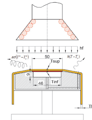
b) Testing method for the new experimental results.
