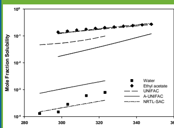
Solubilities of salicylic acid as a function of temperature.
