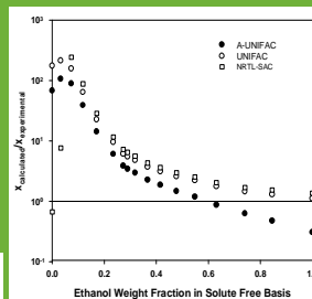
Salicylic acid mole fraction solubility at 298.15 K.
