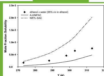
Estradiol mole fraction solubility in ethanol-water mixed solvent.
