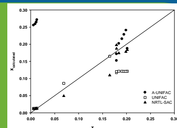
Benzoic acid mole fraction solubility at 298.15 K.
