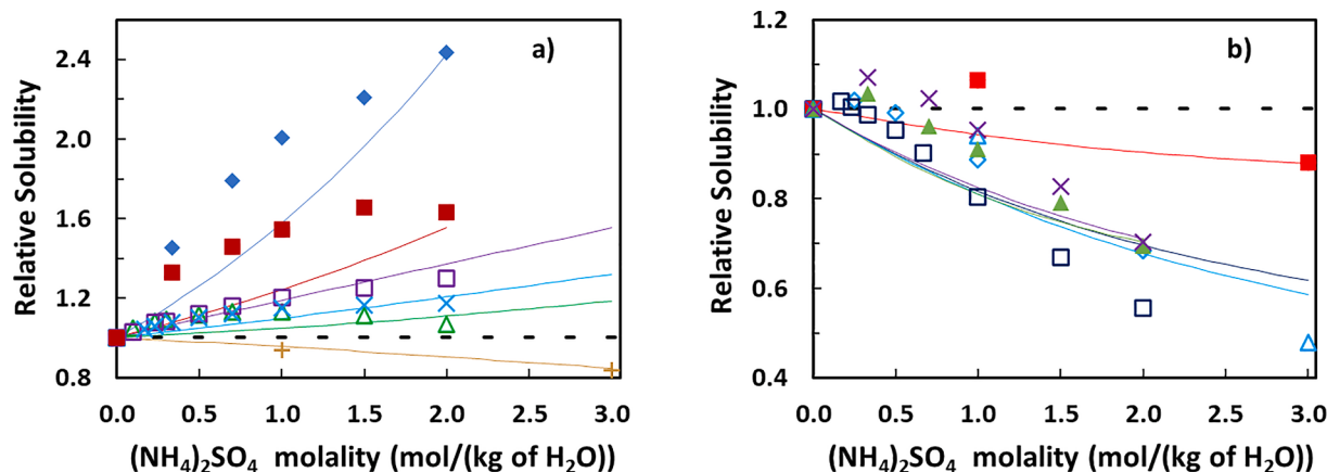
Figure 4. Relative solubility, at 298.2 K, in aqueous solutions of (\text{NH}_4)_2\text{SO}_4 of: a) L-Asp- \blacklozenge (this work); L-Glu- \blacksquare (this work); L-Ser- \square [13]; L-Thr- \triangle [13]; L-Pro- + [18]; Gly- \times [13]; b) L-Trp- \blacktriangle (this work); L-Tyr- \times (this work); L-Ala- \blacksquare [18]; L-Ile- \square [13]; L-Val- \triangle [18], \diamond [14]. Lines were calculated with ePC-SAFT using the parameters from Tables S2, S3 and 4.
