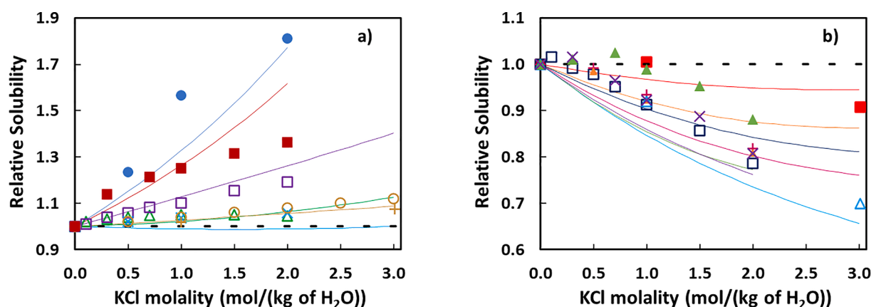
Figure 3. Relative solubility, at 298.2 K, in aqueous solutions of KCl of: a) L-Asp- ● [4]; L-Glu- ■ (this work); L-Ser- □ [12]; L-Thr- △ [12]; L-Pro- ○ [20], + [18]; Gly- ✕ [4]; b) L-Trp- ▲ (this work); L-Tyr- ✕ (this work); L-Ala- ■ [18]; L-Ile- □ [12]; L-Val- △ [18]; L-Leu- ▲ [4]; L-Phe- + [4]. Lines were calculated with ePC-SAFT using the parameters from Tables S2, S3 and 4.
