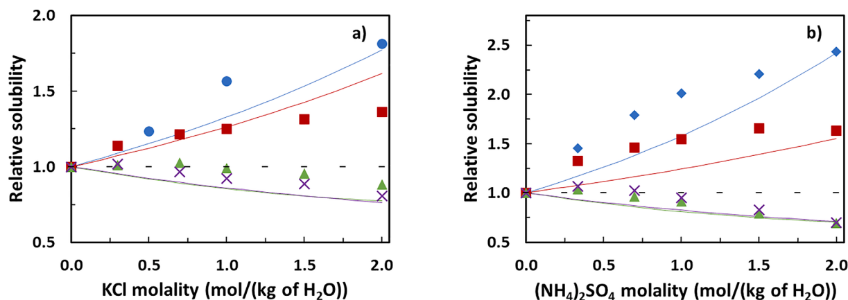
Figure 2. Relative solubility of the amino acids studied in this work in aqueous solutions of KCl (plot a) and (NH 4 ) 2 SO 4 (plot b), at 298.2 K. L-aspartic acid: ● [4] and ◆ (this work); L-glutamic acid: ■ (this work); L-tryptophan: ▲ (this work); L-tyrosine: ✕ (this work). Lines were calculated with ePC-SAFT using the parameters from Tables S2, S3 and 4.
