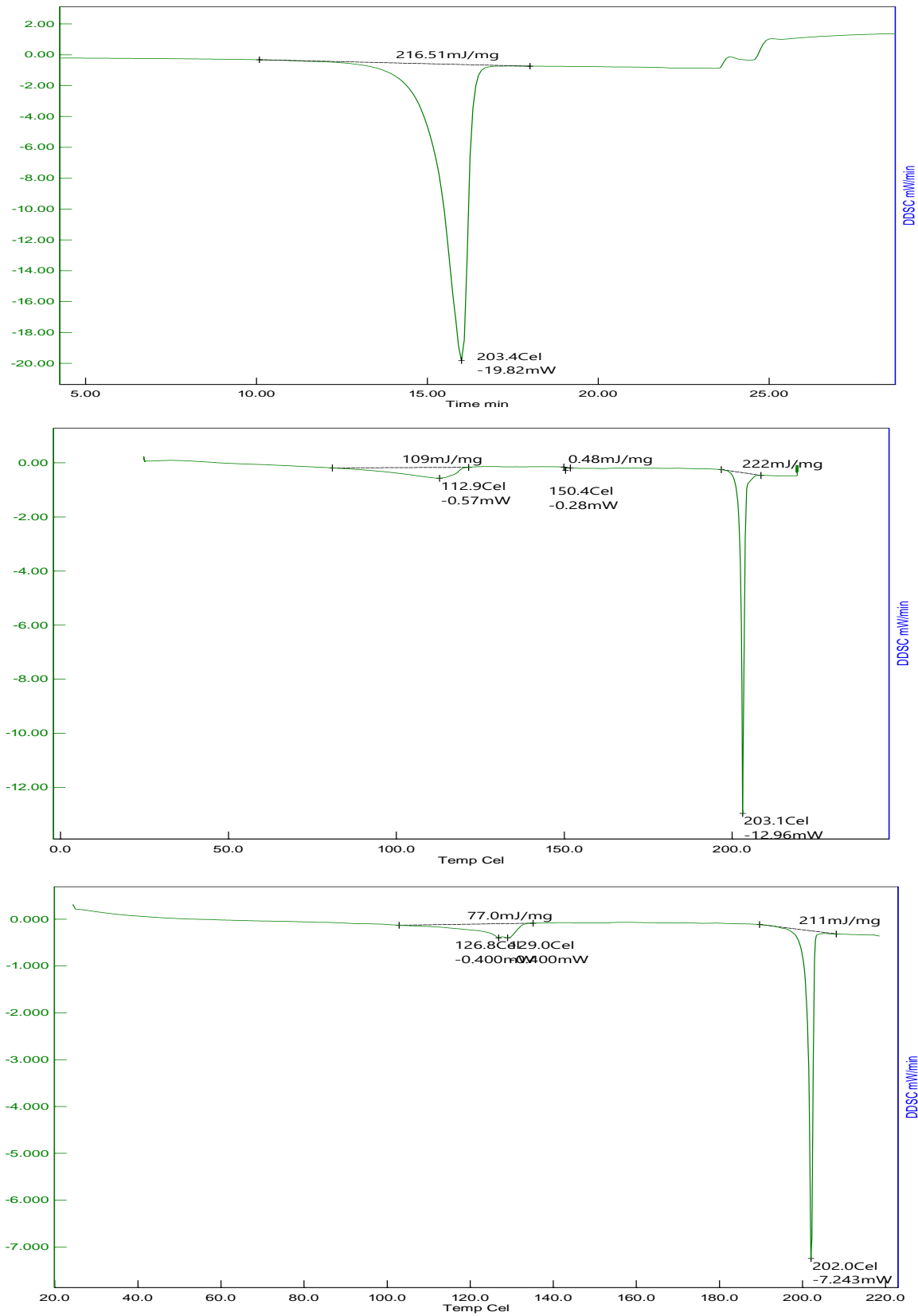
Figure D.2: Thermograms of three DSC analyses performed to protocathechuic acid.
