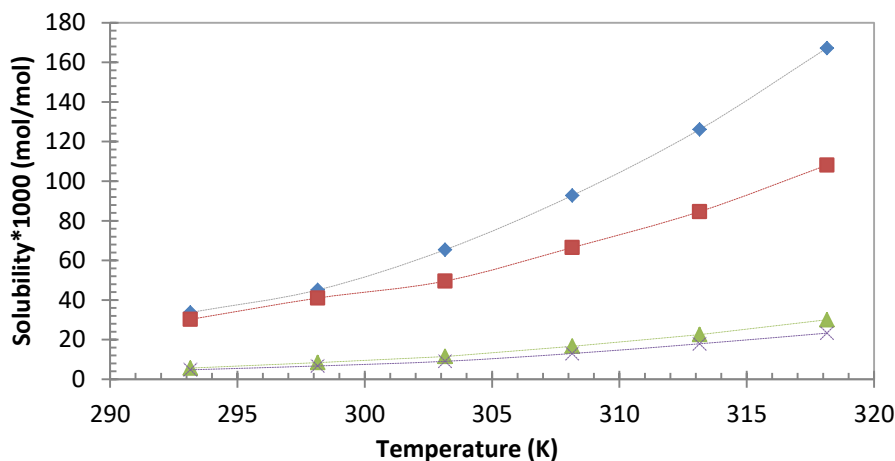
Figure 2.5 Solubility in mole fraction of protocatechuic acid as a function of temperature in different solvents methanol (◆), ethanol (■), methyl acetate (▲) and ethyl acetate (×) (Noubigh et al. 2015).
