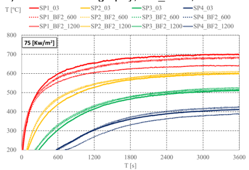
f) Infrared measurements at lateral points (SP1, SP2, SP3 and SP4).
