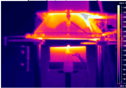
c) Infrared thermography, BF1_1200, t=600 s.
