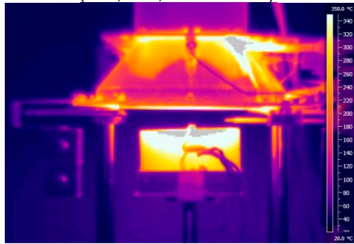
d) Infrared thermography, BF1_1200, t=3600 s.
