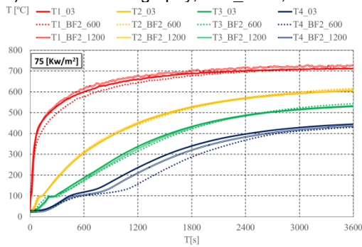
e) Thermocouple measurements at central points (T1, T2, T3 and T4).
