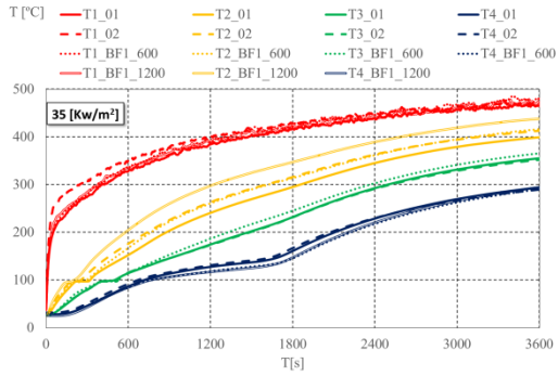
a) Thermocouple measurements at central points (T1, T2, T3 and T4).
