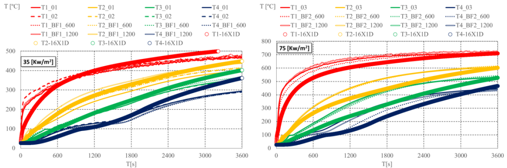
a) Temperature comparison at central points. b) Temperature comparison at central points Figure 7: Temperature comparison using finite difference method.
