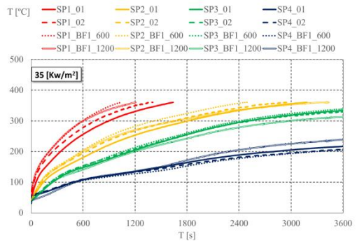
b) Infrared measurements at lateral points (SP1, SP2, SP3 and SP4).
