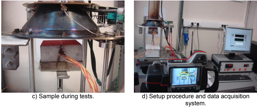
Figure 2: Test model and instrumentation.
