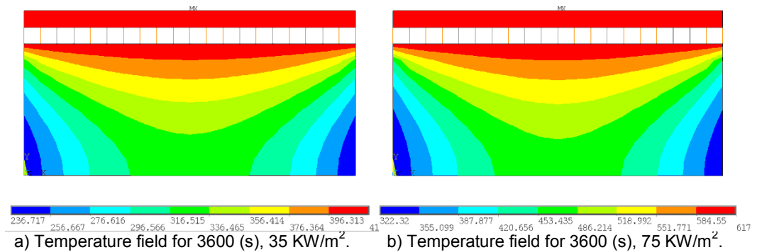
Figure 5 – Temperature field on both samples submitted to 35 and 75 \text{KW/m}^2
