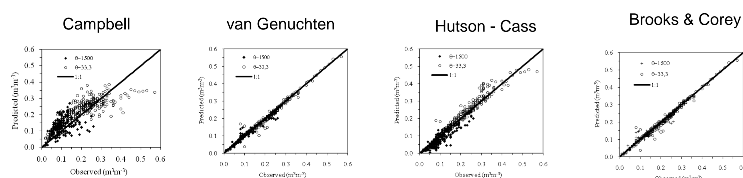
Fig. 3 Predicted versus observed plots of water content at field capacity ( \theta_{-33 \text{ kPa}} ) and permanent wilting point ( \theta_{-1500 \text{ kPa}} ) in relation to the 1:1 line.
