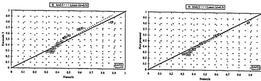
Figure 11: Numerical behaviour, for higher temperatures (above 400[°C]).
