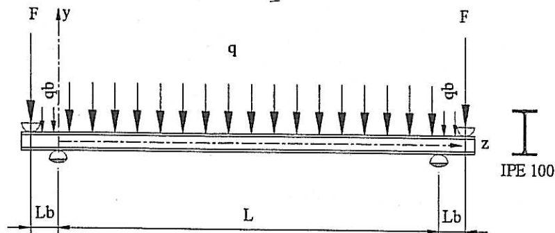
Figure 1: Simple supported beam with tow fork supports.
