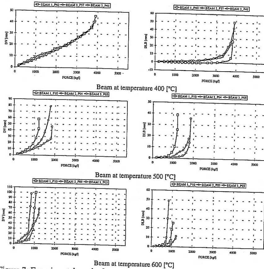
Figure 7: Experimental results from room temperature up to 600 [°C] on a 3.5 [m] span beam.
