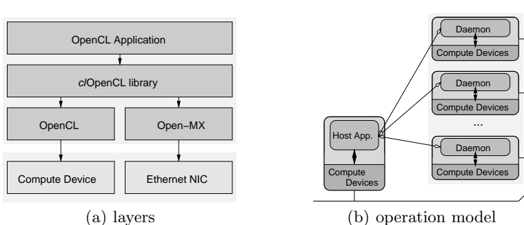
Fig. 1: c/OpenCL architecture.
